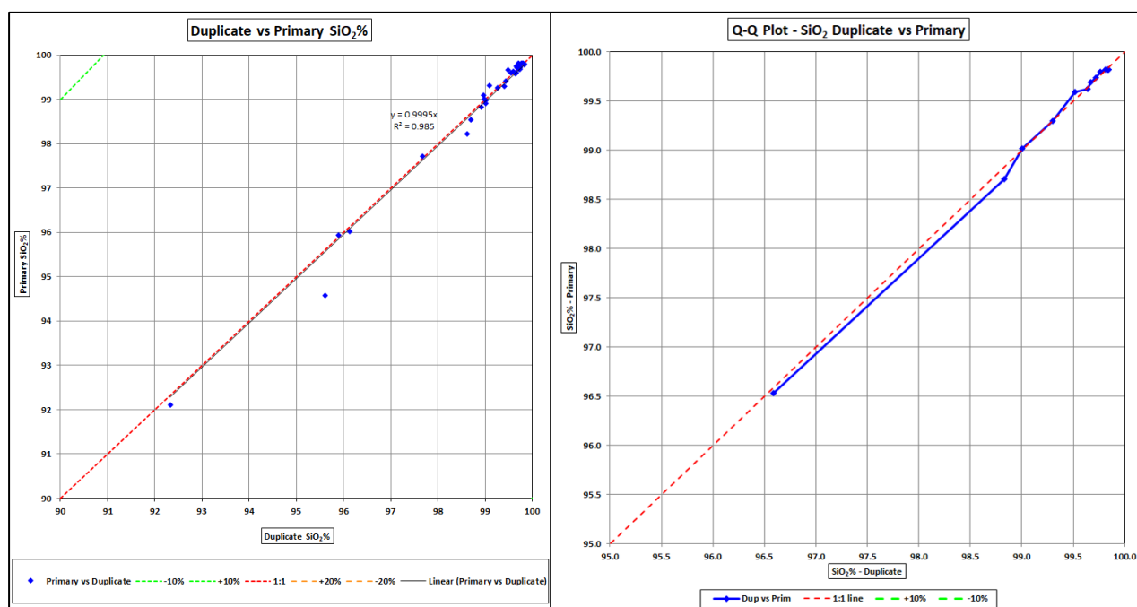
Figure 9: Scatter plot and Q-Q plot Primary vs field duplicate samples for \text{SiO}_2
