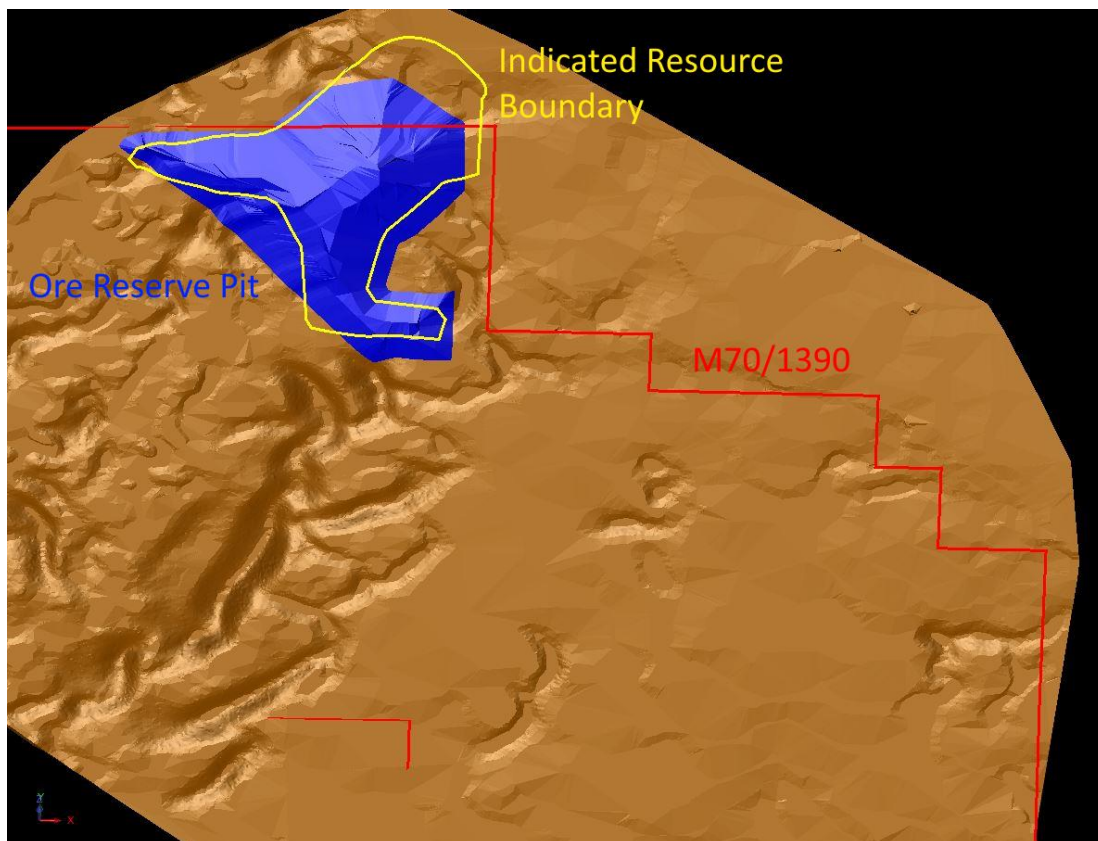
Figure 2: Muchea Pre-Mining Topography (10:1 vertical exaggeration)
