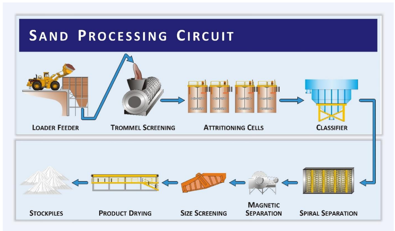
Figure 34: Processing circuit
