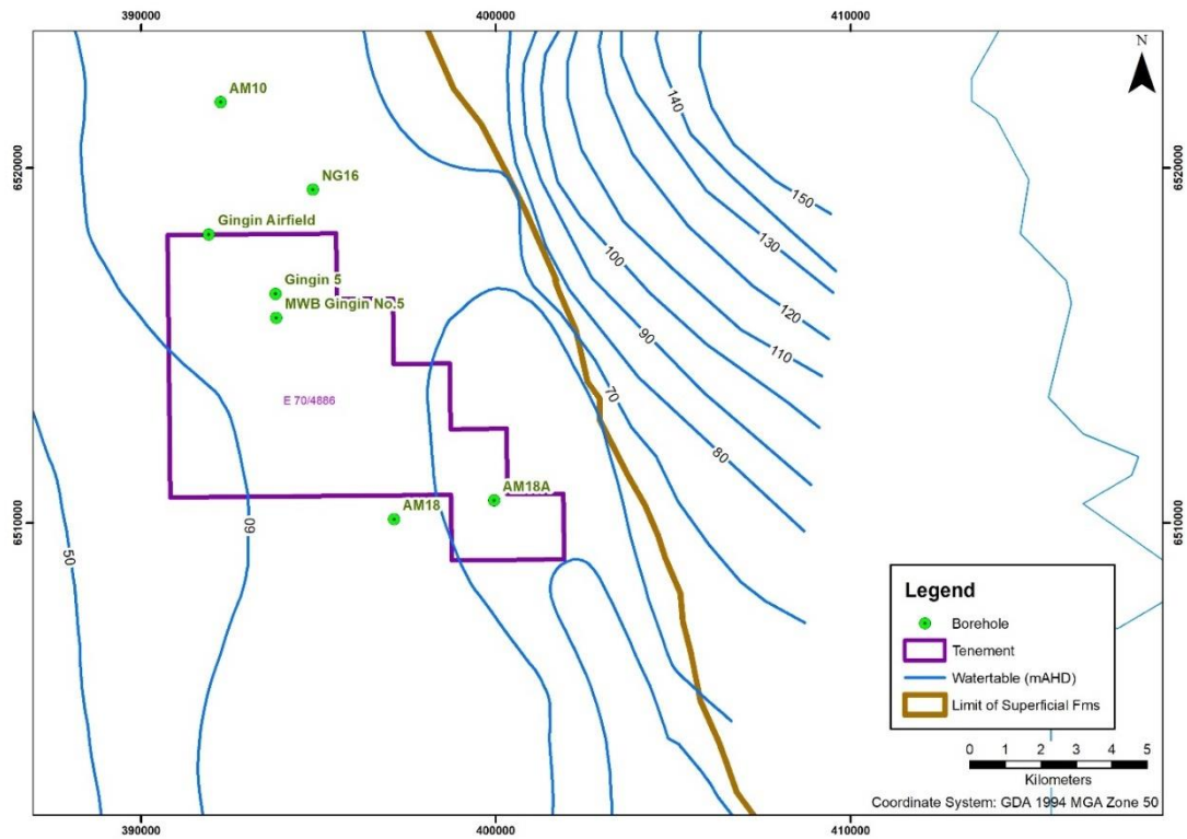
Figure 43: Watertable elevation.
