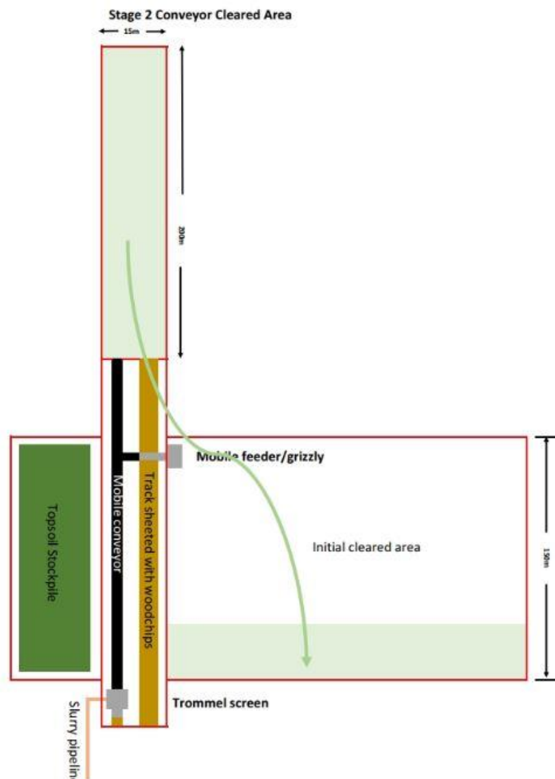
Figure 18: Mining process – conveyor cleared area
