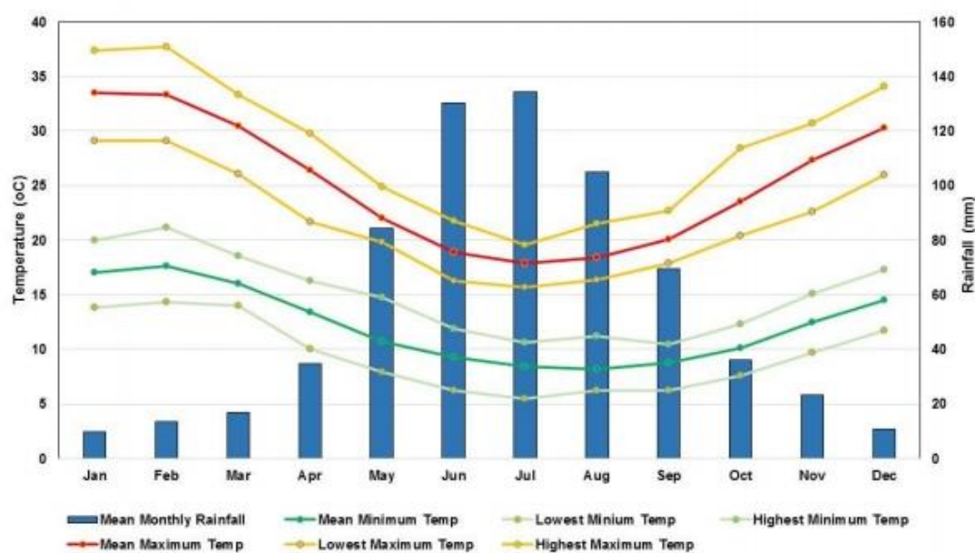
Figure 2: Rainfall and temperature data for Pearce Airbase (SE of the Project area)
