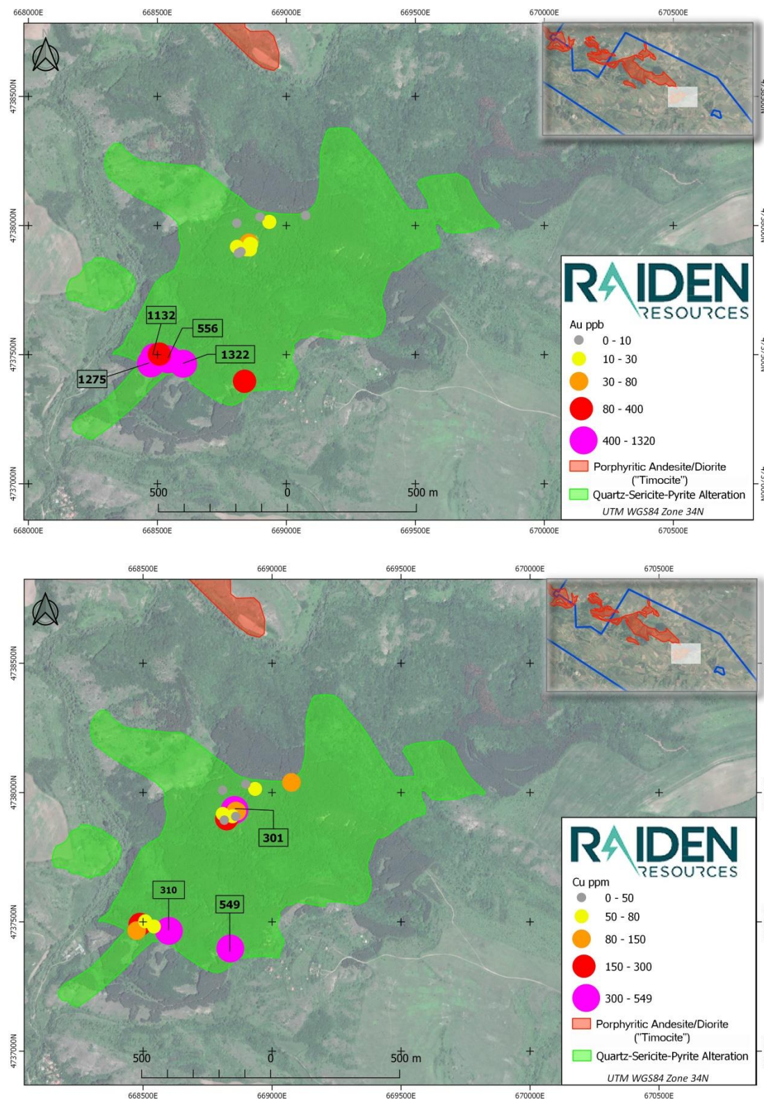
Figure 2: Rosoman Prospect quartz-sericite-pyrite (phyllic) alteration mapping and the results of QX's limited reconnaissance outcrop sampling program. The diagrams show gold (top) and copper (bottom) concentrations. The prospect is defined by a 1.5 km x 1 km zone of intense alteration. The results demonstrate that the phyllic alteration zone coincides with elevated concentrations of gold and copper.
