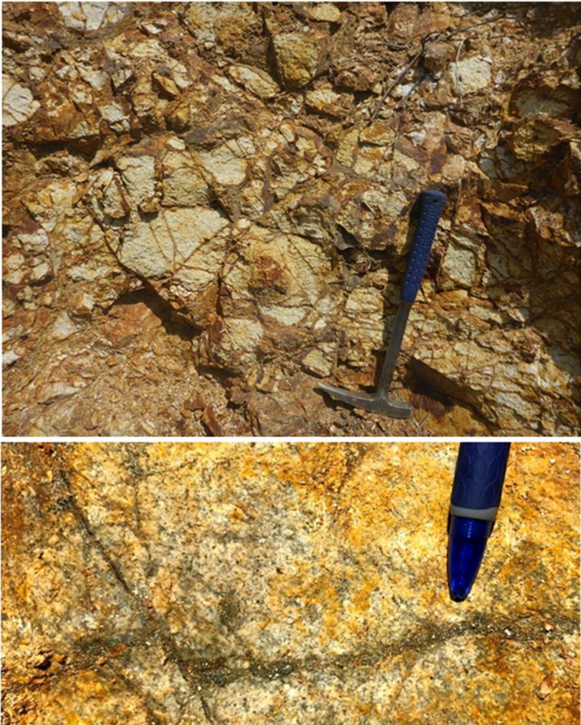
Figure 4: Outcrops in the Rosoman prospect. Top: Limonite (likely after pyrite) stockwork. Bottom: Quartz-pyrite veining and disseminated pyrite in porphyritic diorite
