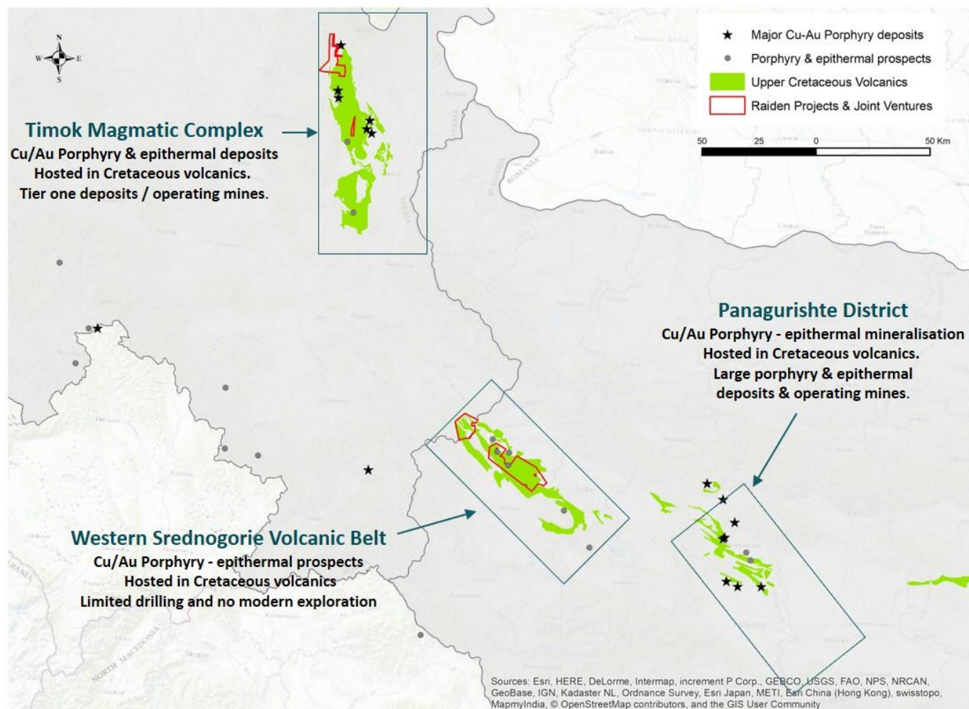
Figure 6: Location of the Donje Nevlje project (100% Raiden) and the Zlatusha joint venture project. Raiden has a commanding position within the Western Srednogorie belt. In comparison to the Panagurishte and the Timok districts, the middle belt remains under-explored and presents the Company with an opportunity to make a considerable discovery
