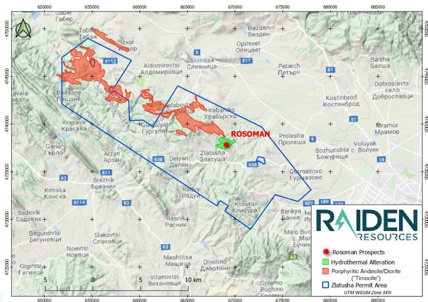
Figure 1: The location of the Rosoman Prospect in the Zlatusha permit area. The prospect was first defined when Bulgarian State agencies mapped a 1.4 km 2 zone of intense hydrothermal alteration. The zone occurs adjacent to sub-volcanic porphyritic andesites and diorites, referred to in the literature as "Timocite" and shown in red. It is important to note that in the Timok Magmatic Complex and the Panagyrishte Belt (see also Figure 6) along strike to the northwest and southeast of Zlatusha, all major copper and gold deposits are spatially associated with Timocite
