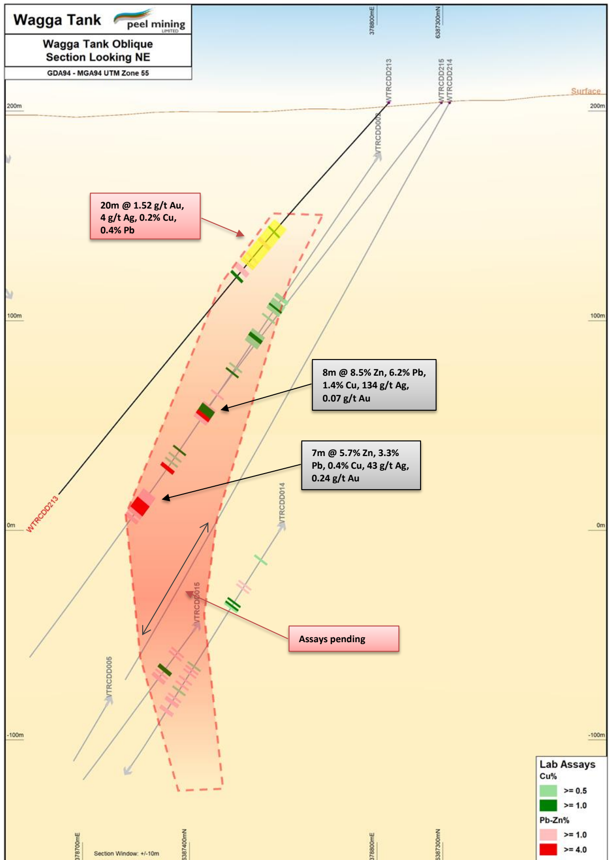
Figure 4 – Wagga Tank Cross Section
