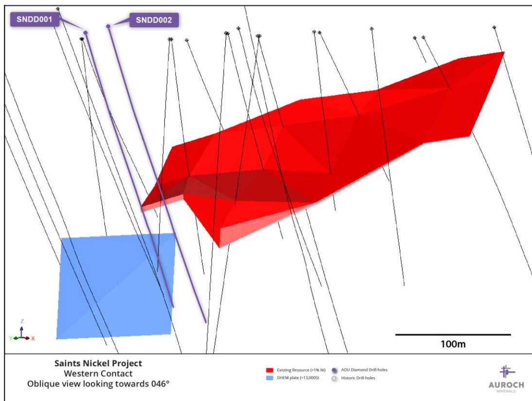
Figure 2 – a) Plan view and b) Oblique view of the Western Contact (looking towards 046°) of the Saints Nickel Project showing the very strong modelled EM plate (>13,000S) and the location of drill-holes SNDD001 and SNDD002 in relation to known high-grade nickel sulphide mineralisation (1.0% nickel cut-off wireframes shown in dark red).
