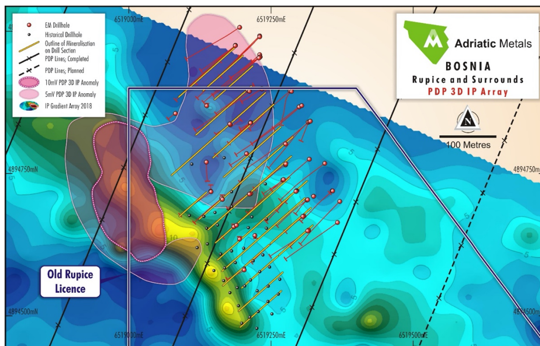
Figure 2 - PDP3D IP Response over and to the West of the Rupice Mineralisation
