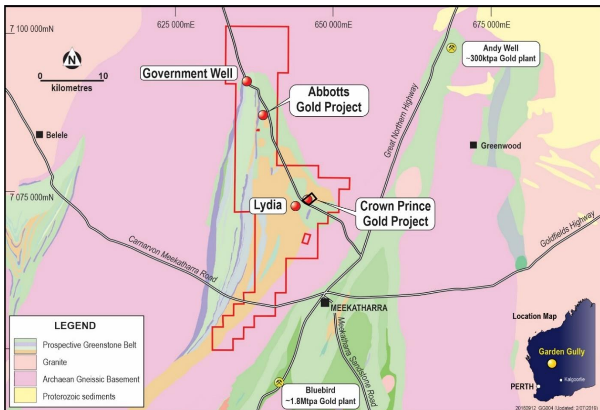
Figure 1. Government Well location with Ora Gold tenements, regional geology and main projects
