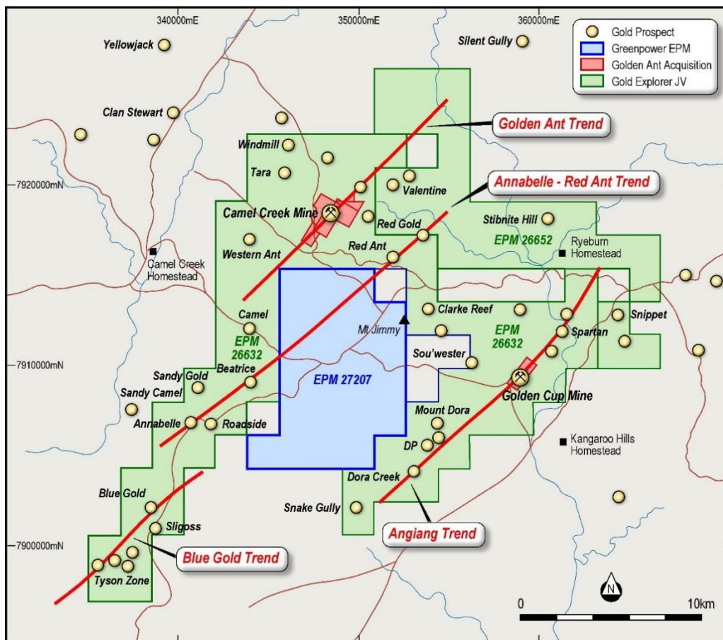
Figure 1: Location of new Gold Explorer JV exploration permits complementing the current Camel Creek and Golden Cup Projects
