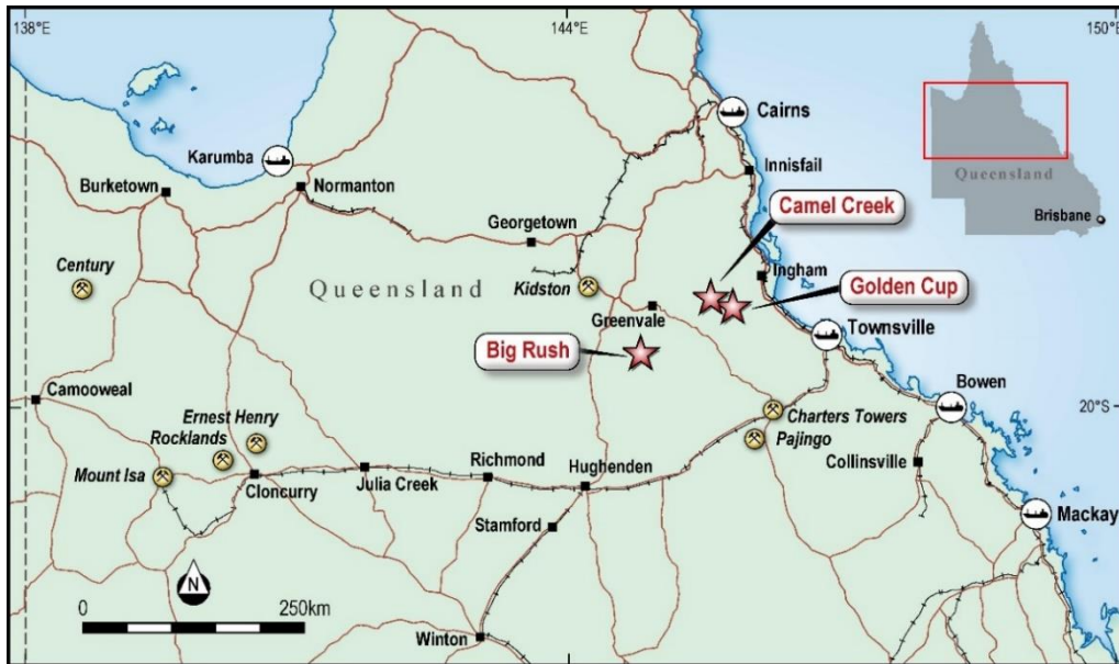
Figure 2: Location of Greenpower's Camel Creek, Golden Cup & Big Rush gold projects
