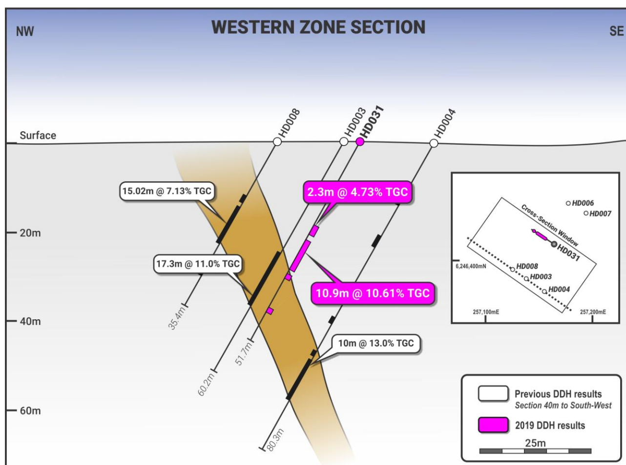
Figure 1. Schematic cross section looking north-northwest showing consistent high-grade graphite in HD031 projected onto previous drilled and interpreted section 6246380N, 40m south of new hole.
