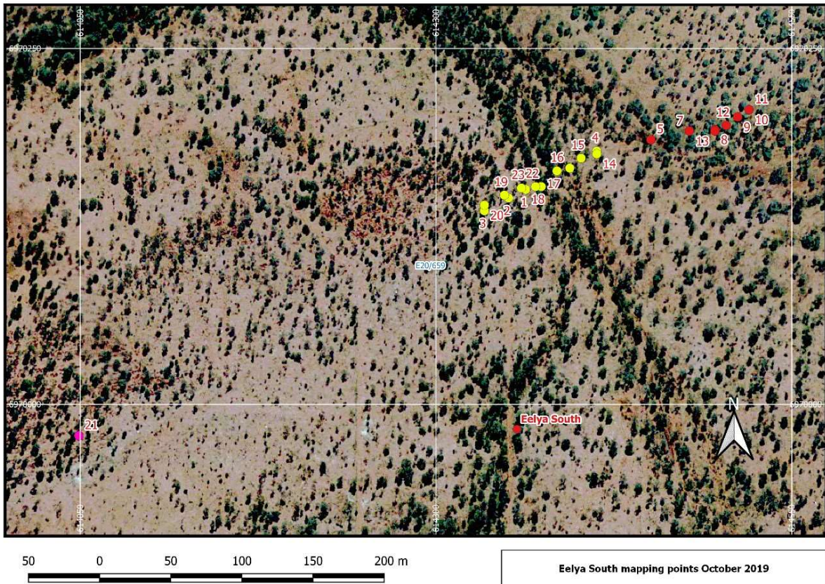
Figure 3 / Mapping points of the Elya South outcropping shear hosted mineralisation
