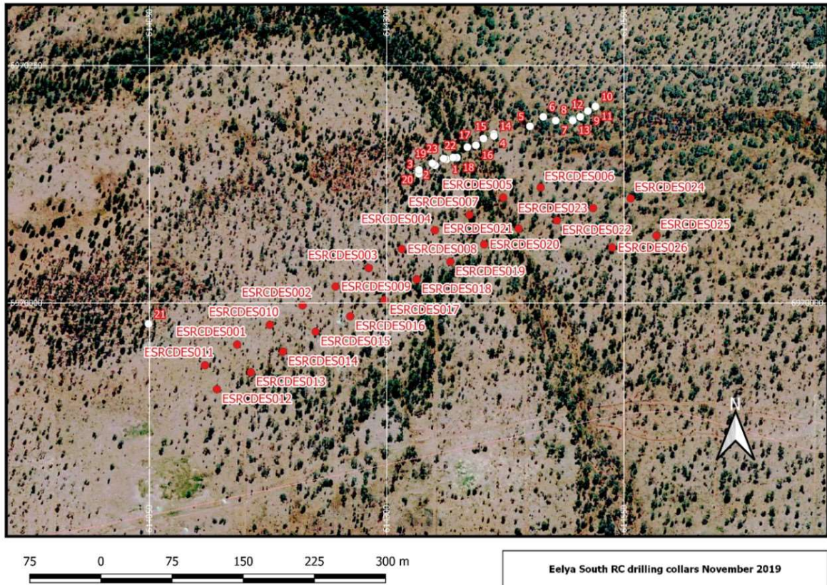
Figure 1 / Eleya South November 2019 drilling programme collar locations
