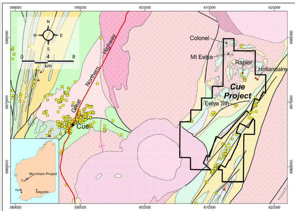
Figure 2 | Location of Eleya South at the Cue Copper Project tenements
