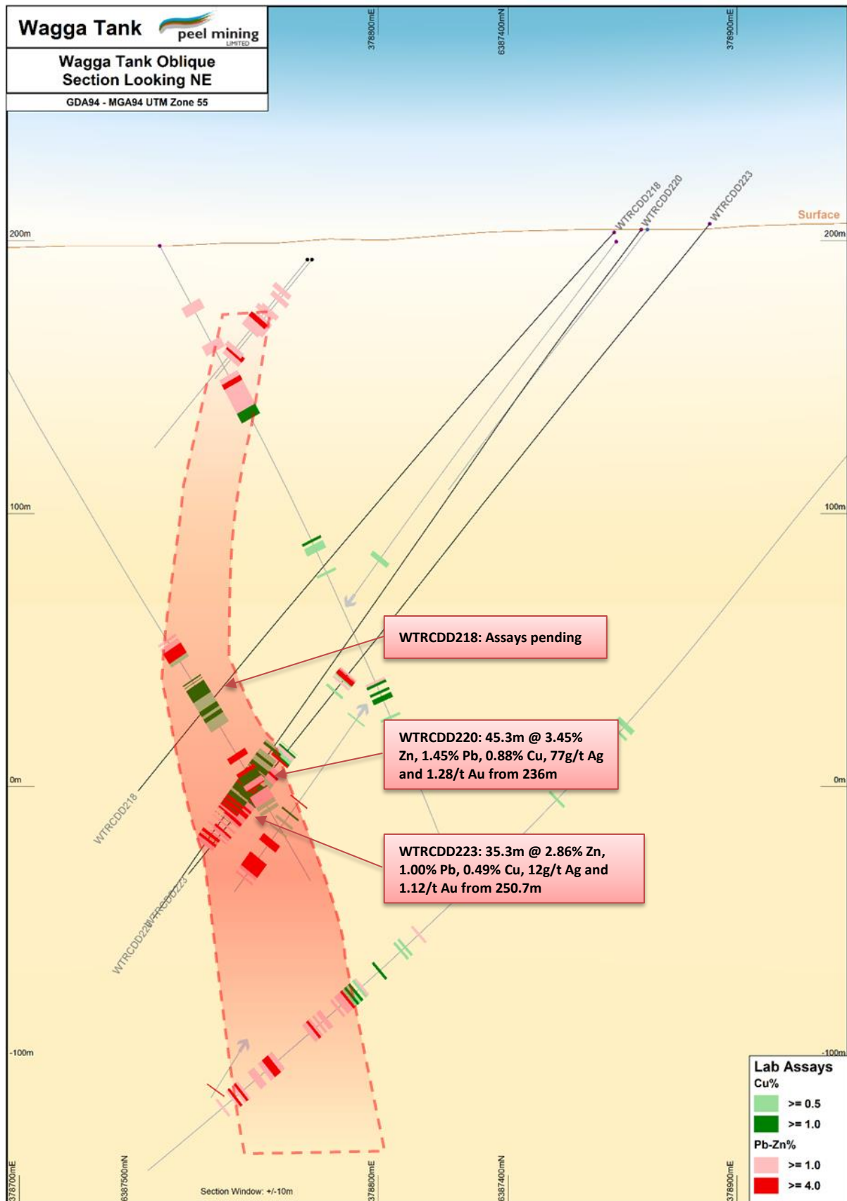
Figure 5 – Wagga Tank Cross Section 1 (WTRCDD220 and WTRCDD223)
