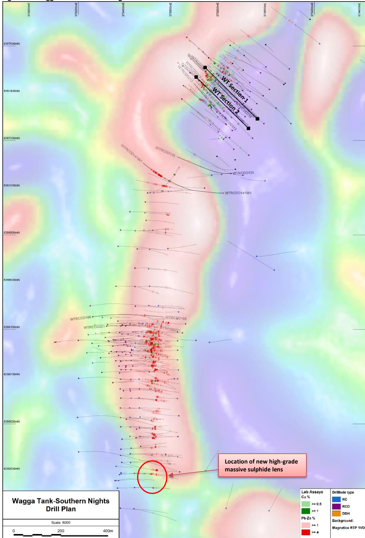
Figure 3 - Wagga Tank-Southern Nights Drill Plan
