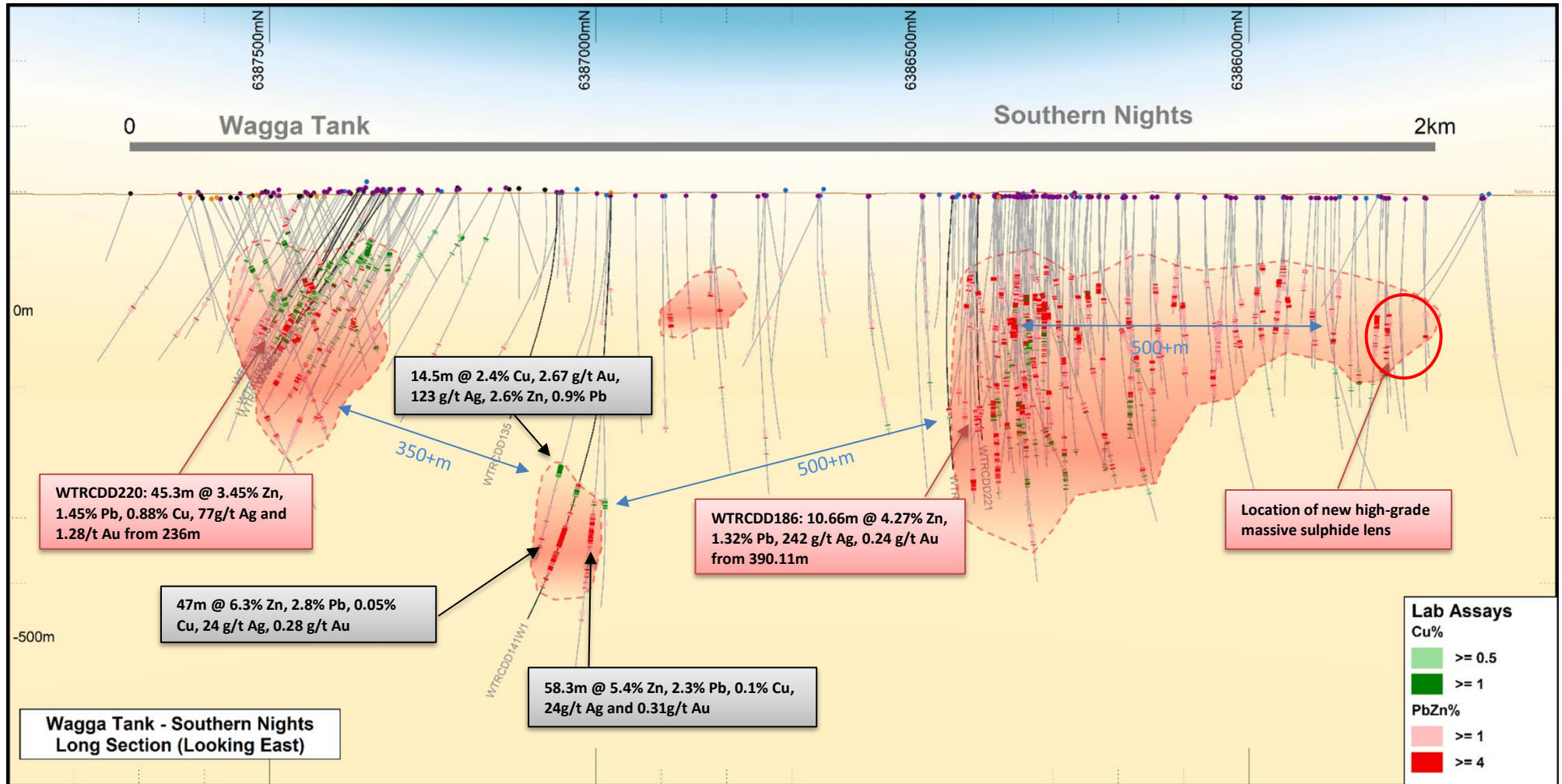
Figure 4 – Wagga Tank-Southern Nights Long Section
