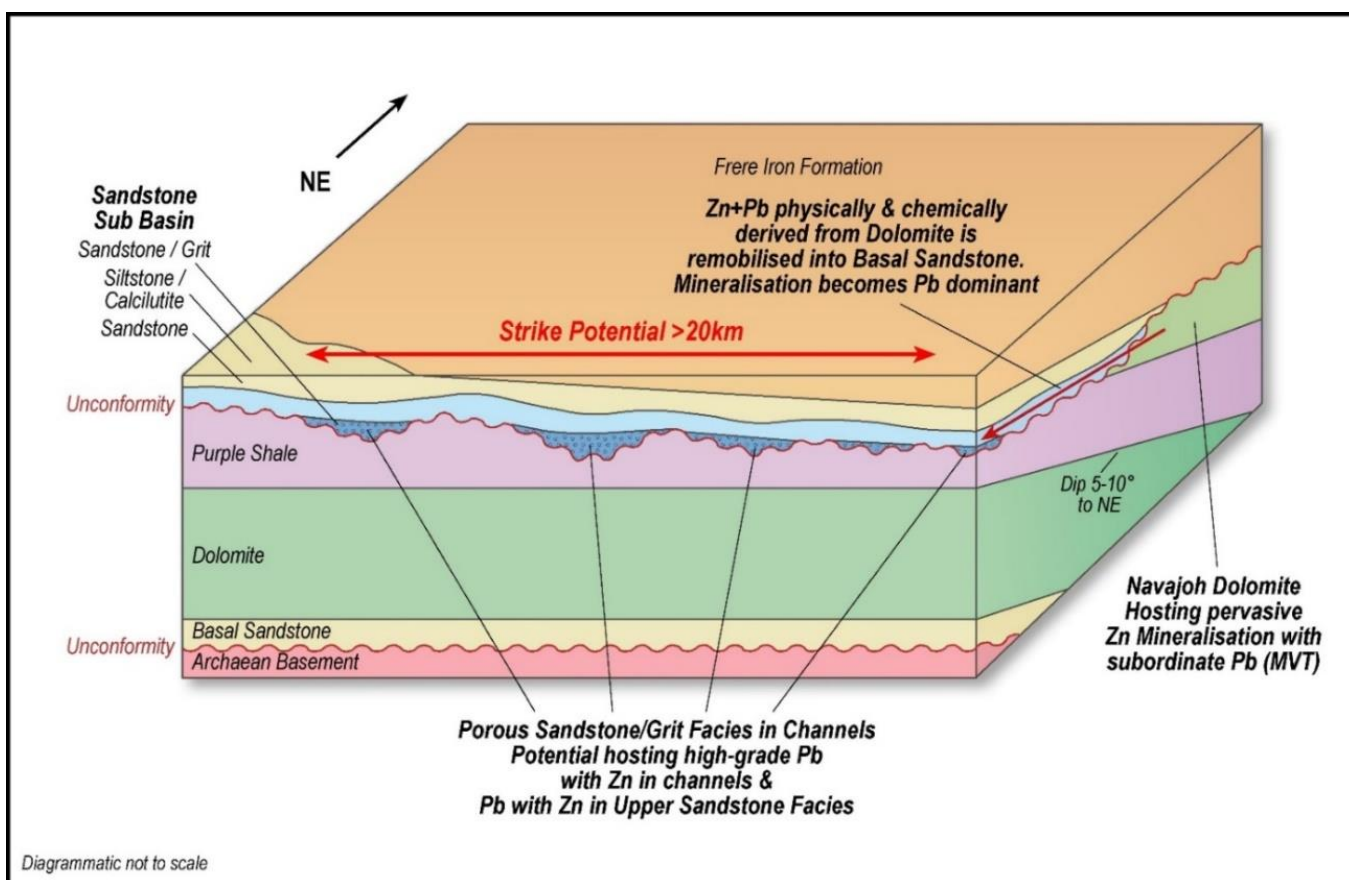
Image 9 – Geological Model for Sandstone Hosted Zn - Pb Deposits (Earacheedy Project)
