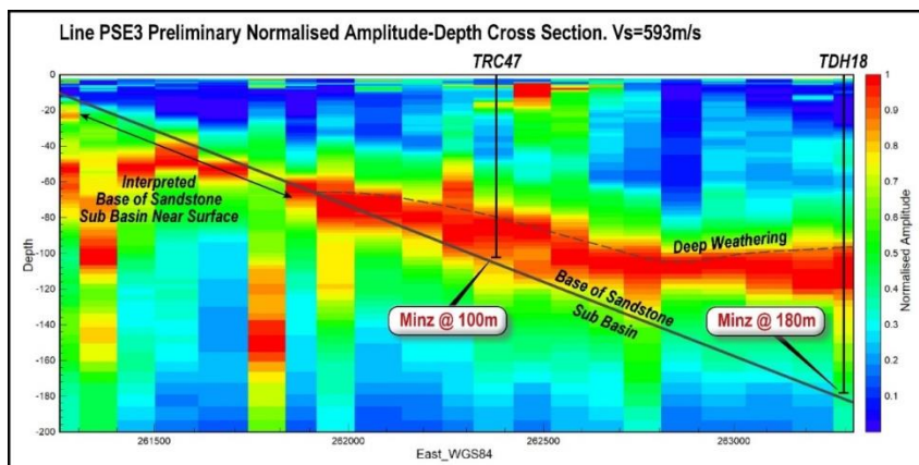
Image 7 – Passive Seismic Traverse PSE3 with Interpretation – Note Dip of Sandstone is 5-10°NE
