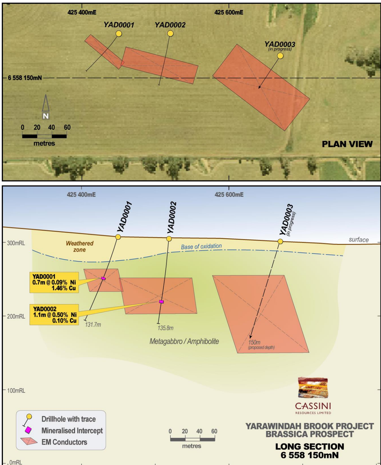
Figure 2. Long section and location plan of drilling at the Brassica Prospect.
