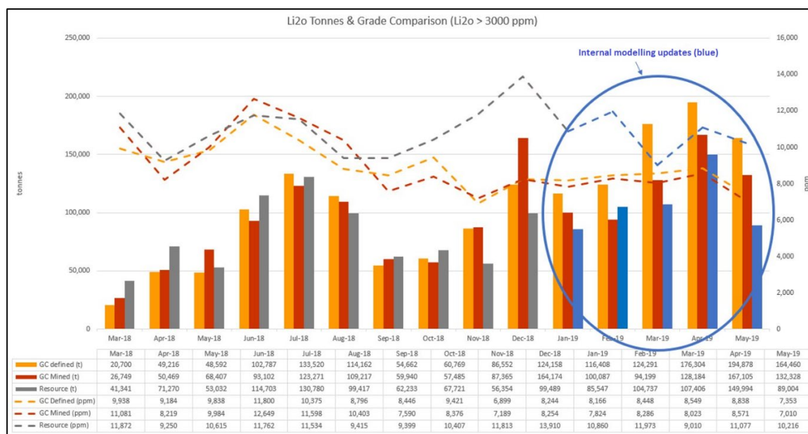
Figure 3-6: Mining production summary
