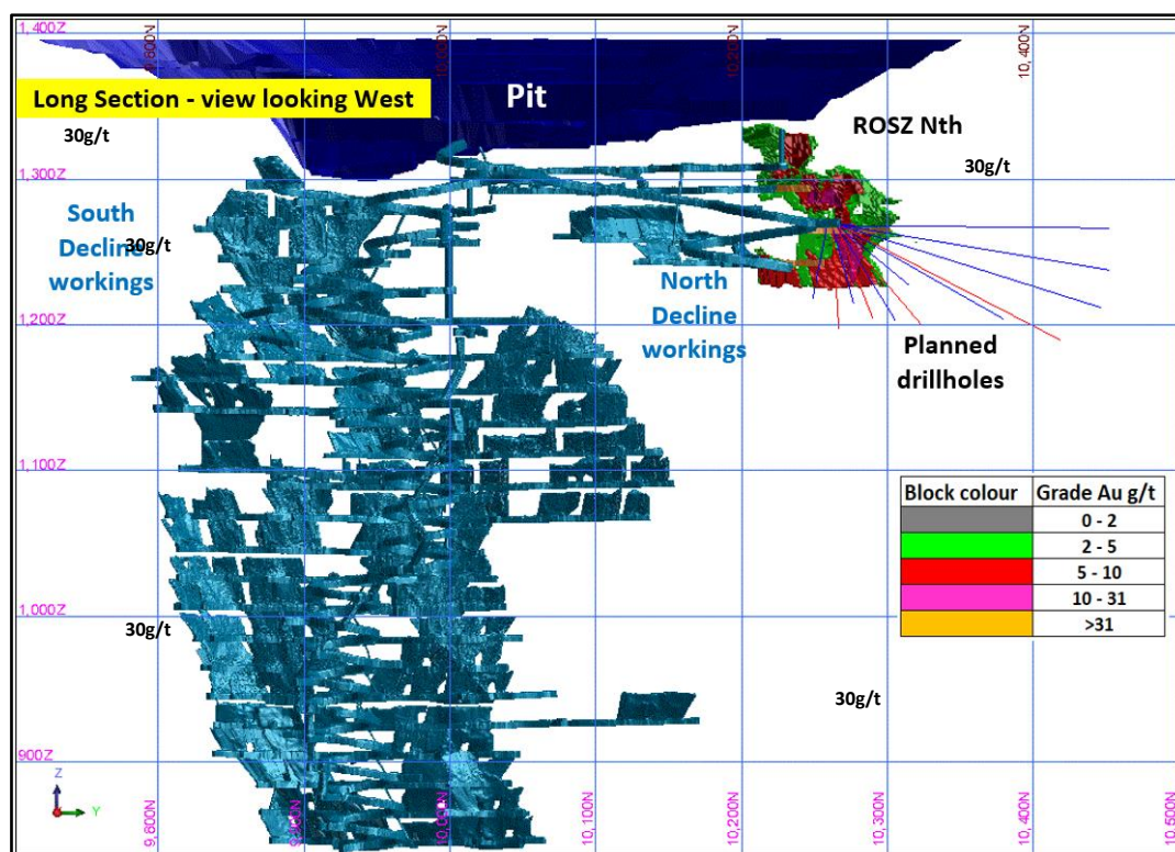
Figure 4: Long Section view - mine workings, grade control block model ROSZ (>3g/t), planned drillholes
