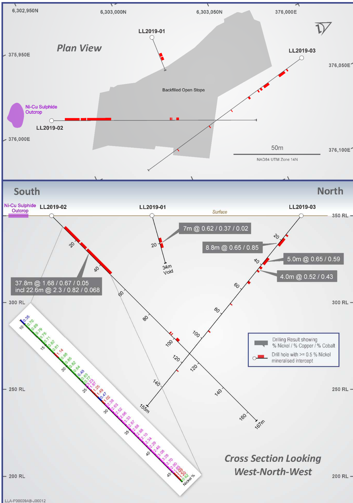
Figure 2 – A Orebody drill hole location plan and cross section
