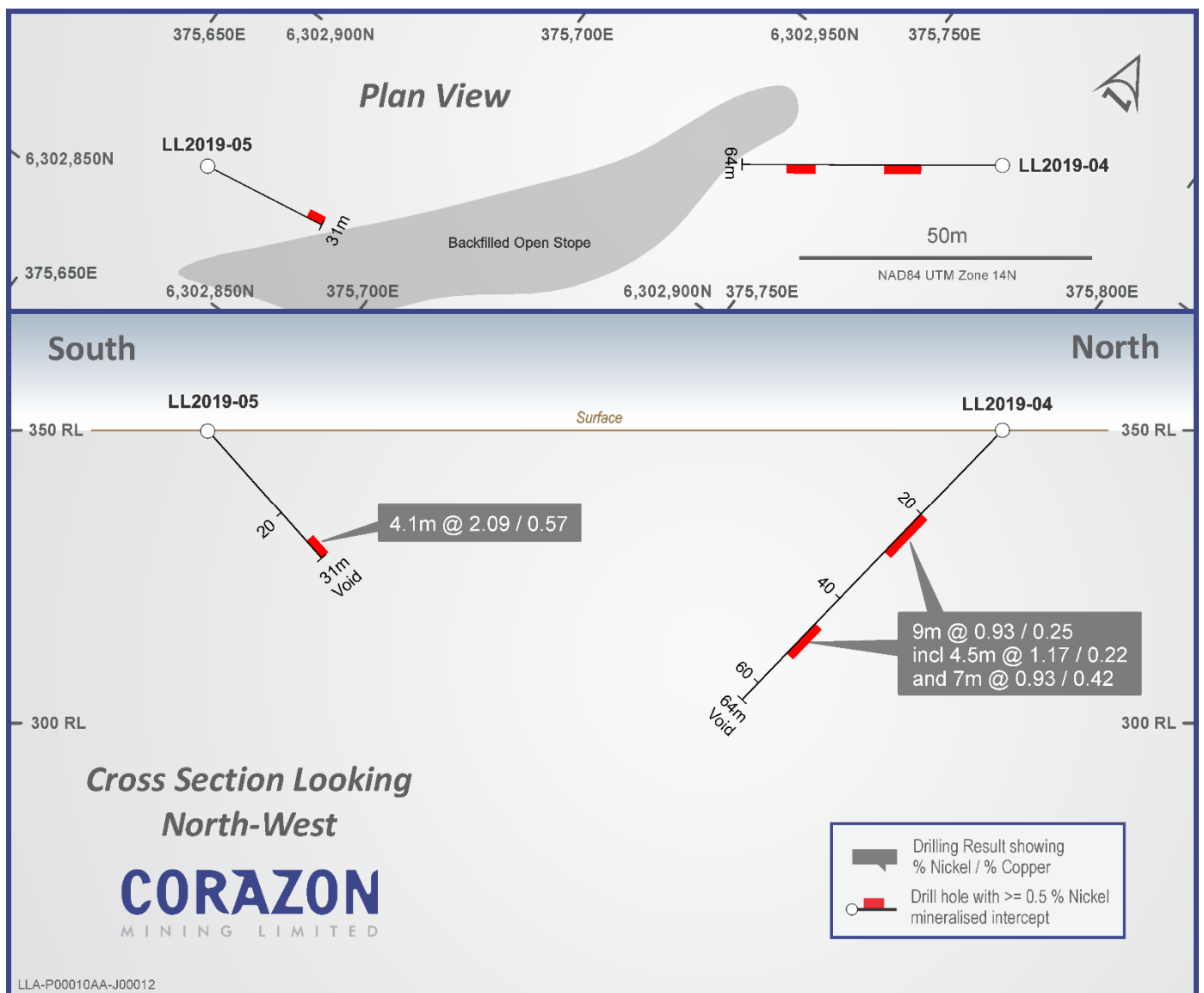
Figure 3 – E Orebody drill hole location plan and cross section
