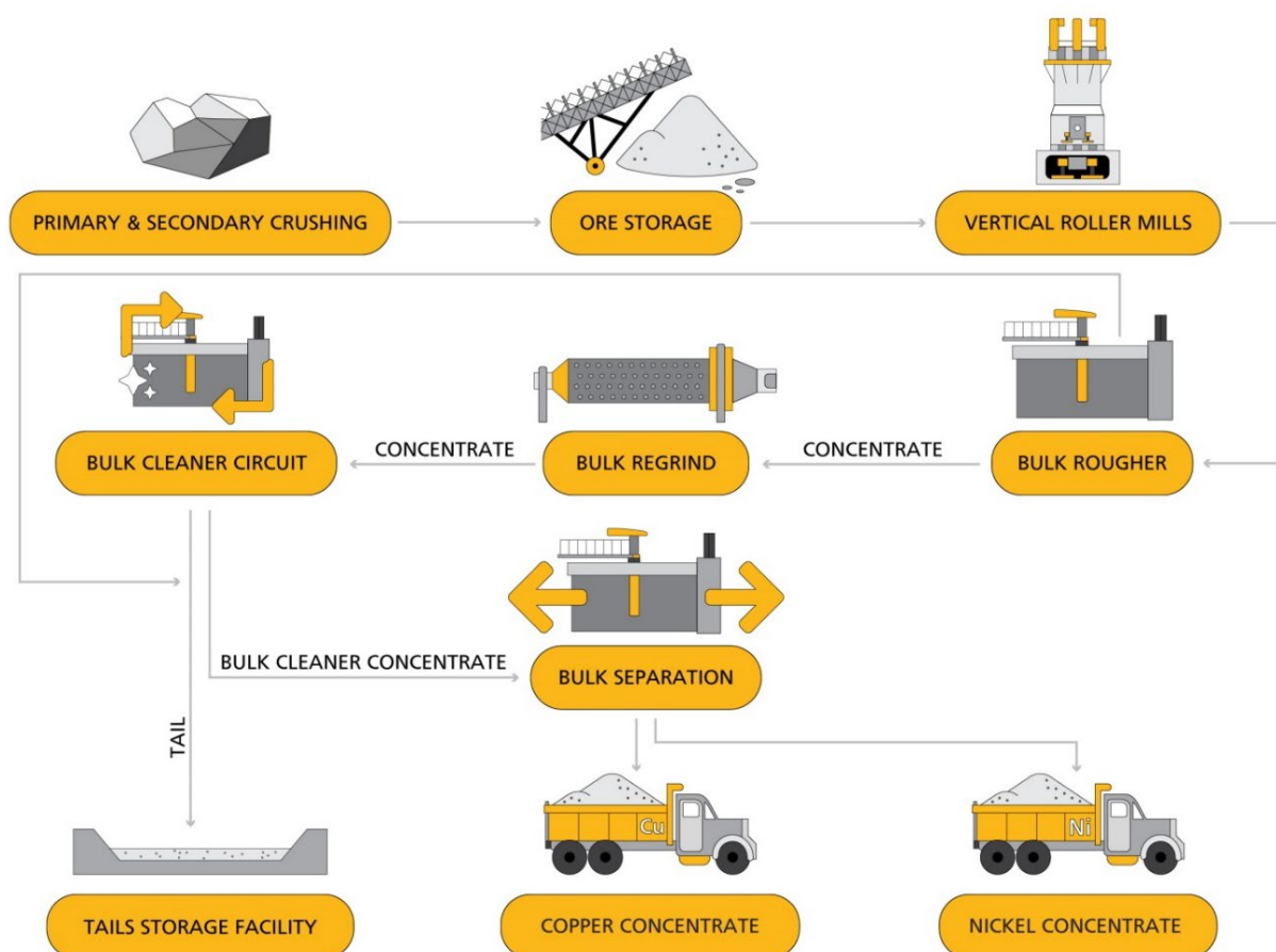
Figure 4: Process Flowsheet
