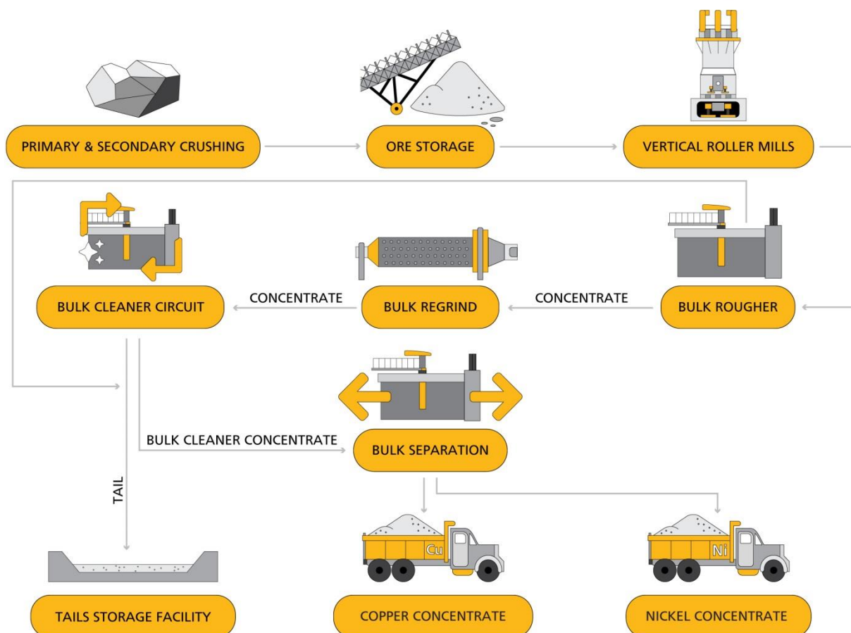
Figure 2: Flowsheet
