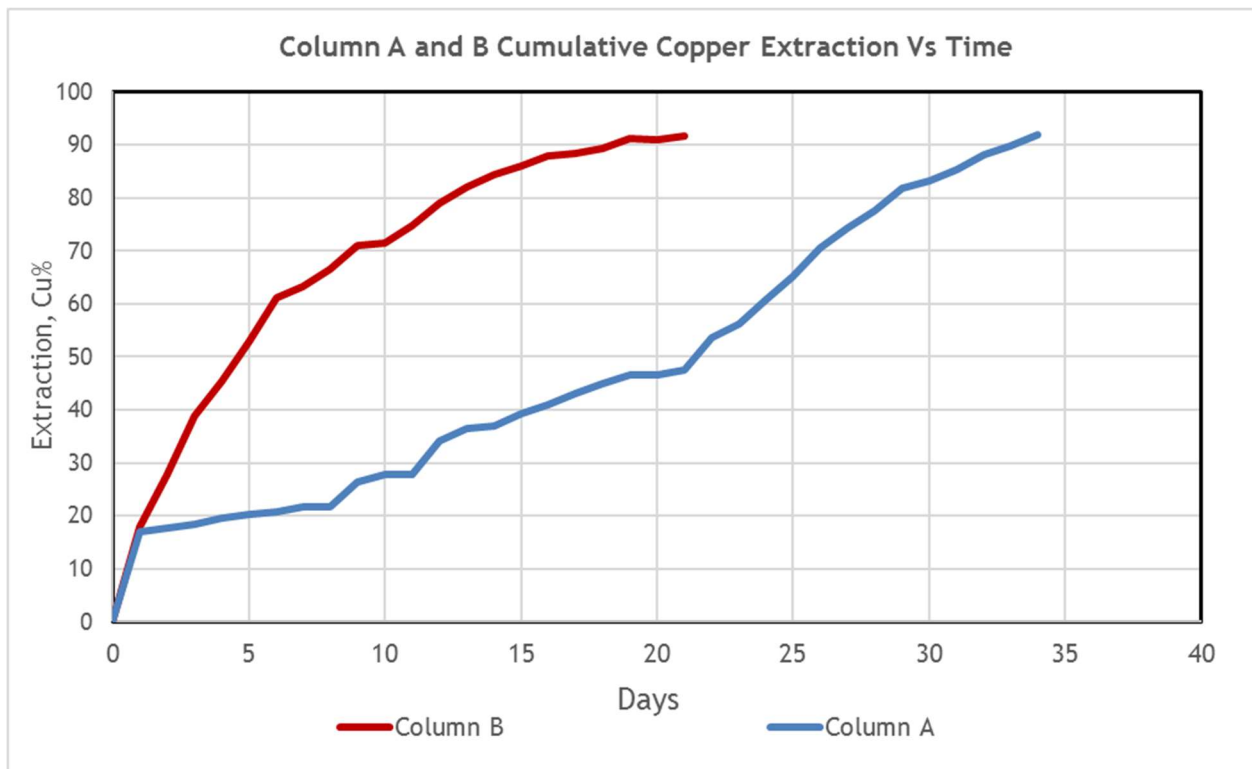
Graph 1 / Copper Extraction
