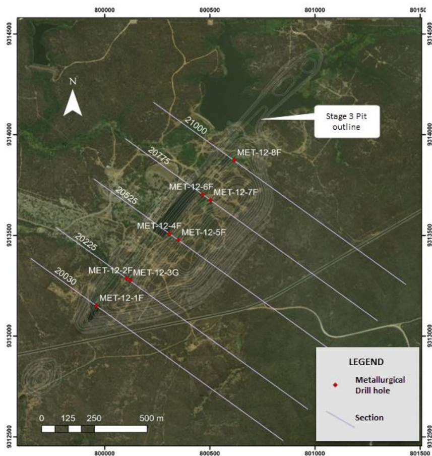
Figure 3. Location of metallurgical drillholes drilled in along the Borborema ore zone within the original Stage 3 planned open pit.
