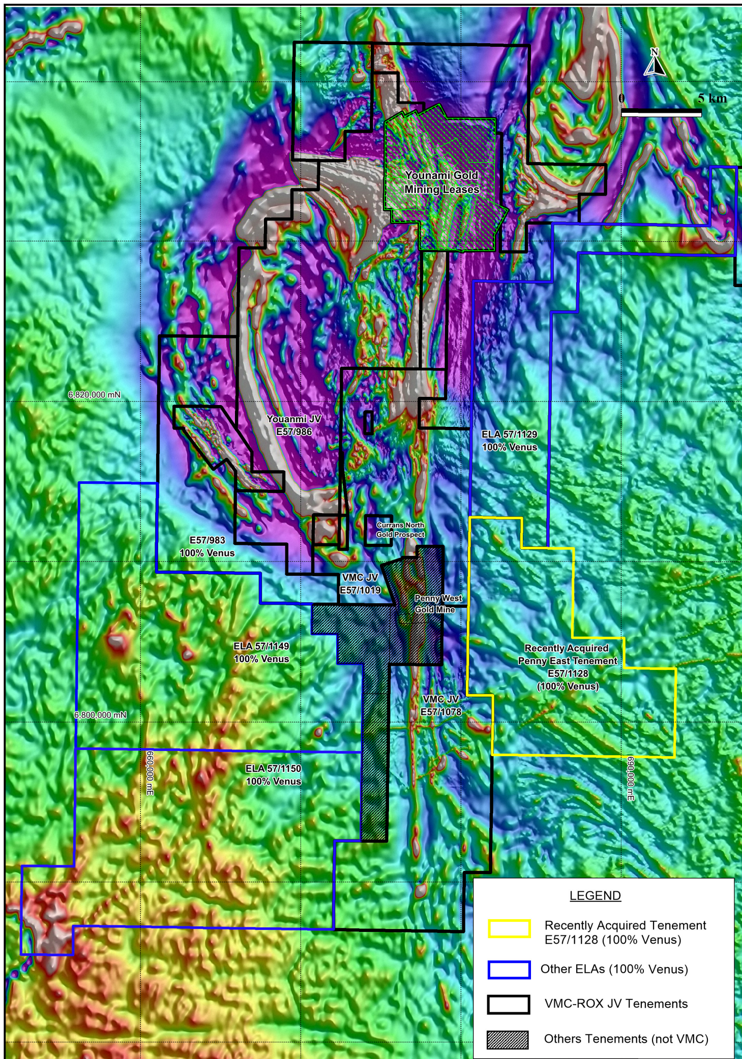
Figure 1. Location of Venus's recently acquired Penny East tenement (E57/1128) and other ELAs at the Youanmi Gold Project on regional aeromagnetic image
