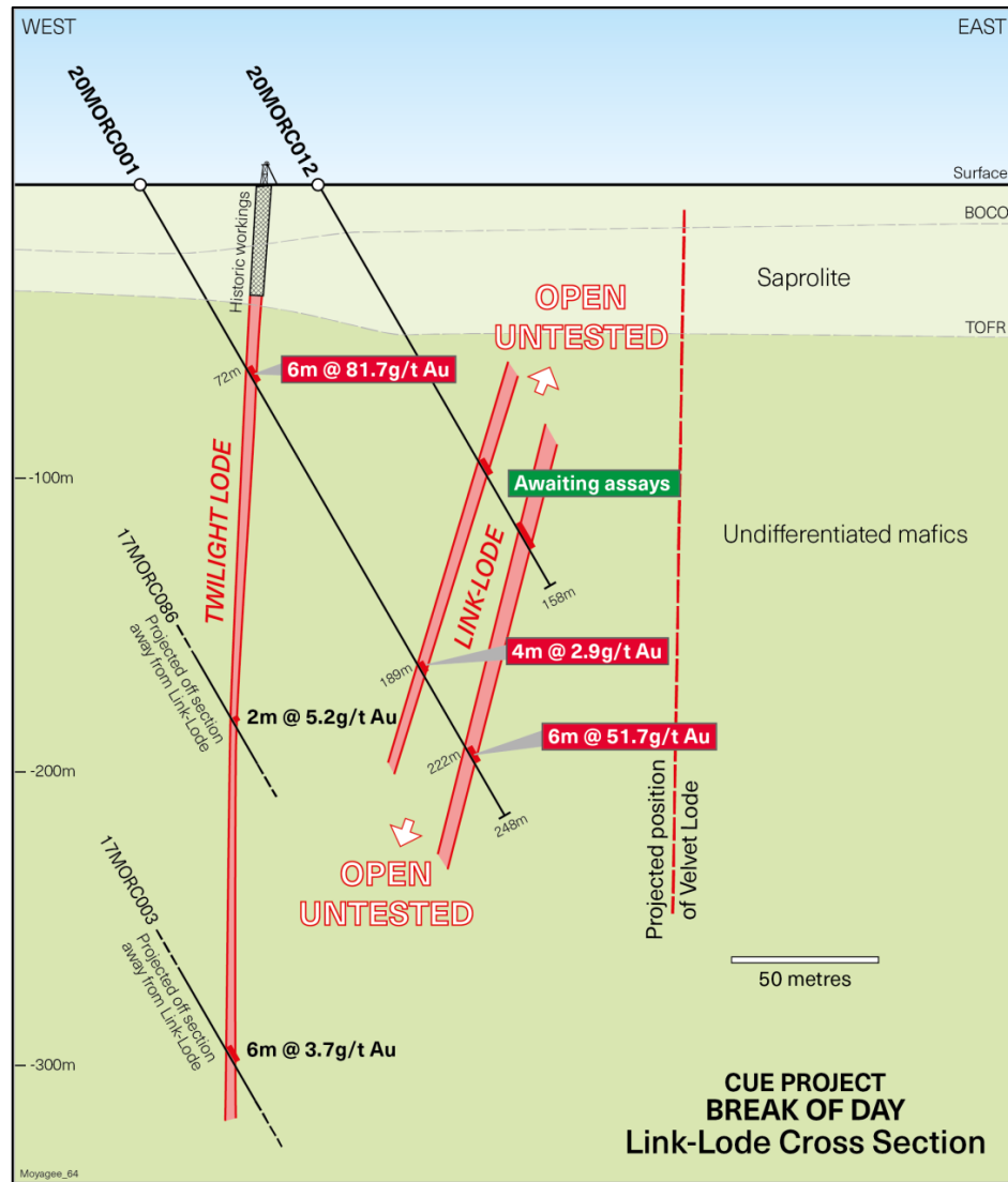
Figure 3: Cross-section of new Link-lode at Break of Day
