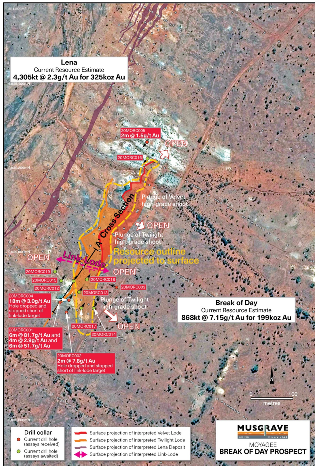
Figure 2: Plan showing Link-lode position at Break of Day and new drill collars and assay results
