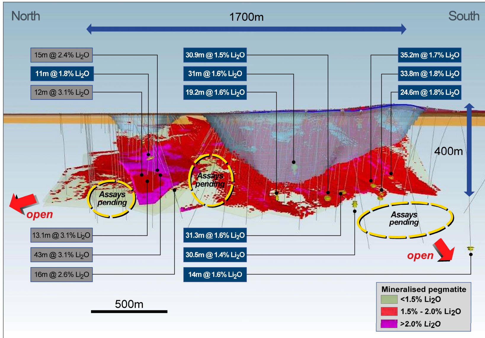
Figure 1: Kathleen Valley – 3D image showing high grade (>1.5% Li 2 O) blocks within block model for recent MRE update and latest drill intersections.
