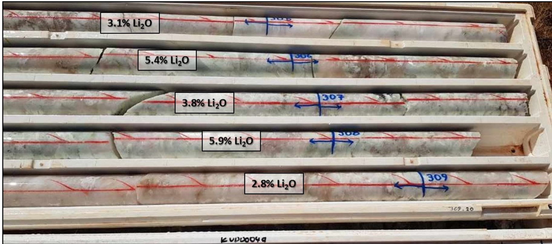
Figure 2: Kathleen Valley – Drill core showing spodumene-rich pegmatite from hole KVDD0048 304.5 – 309.2m.
