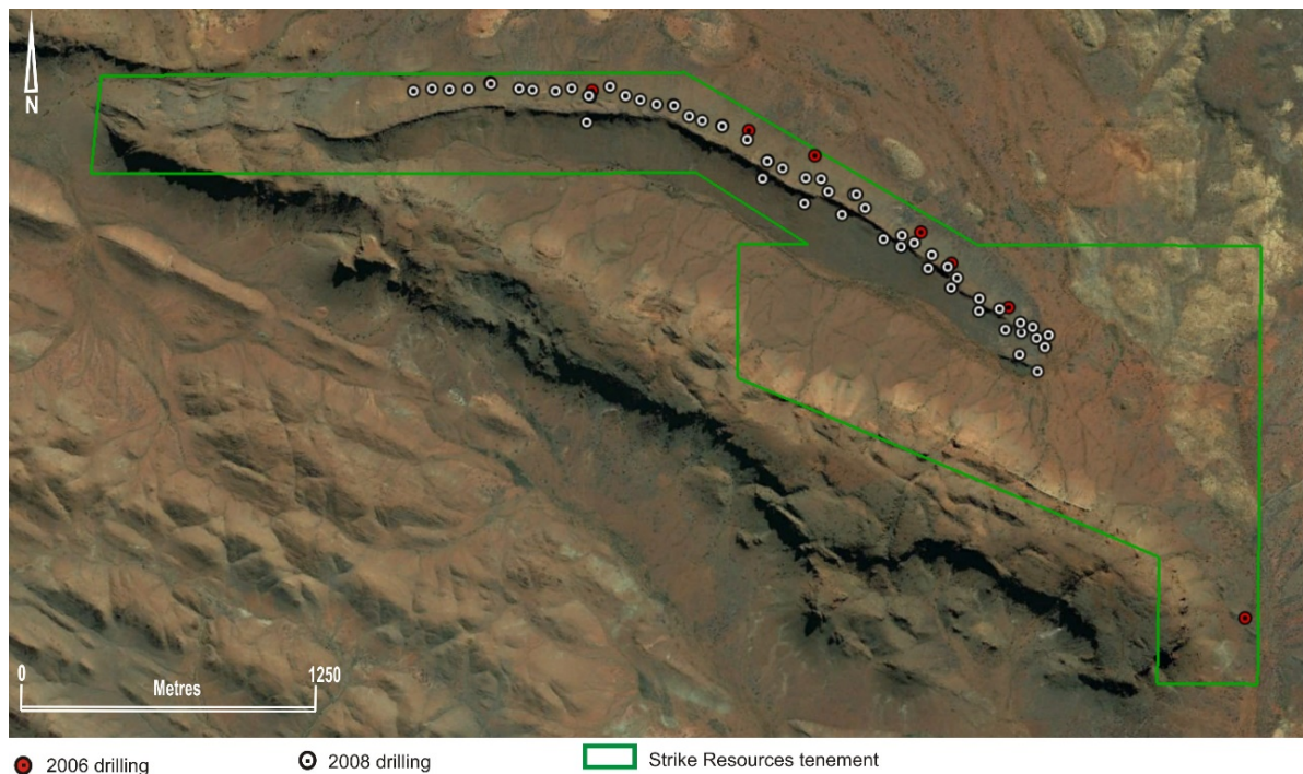
Figure 20: Drill hole location plan showing semi-regular spacing of holes
