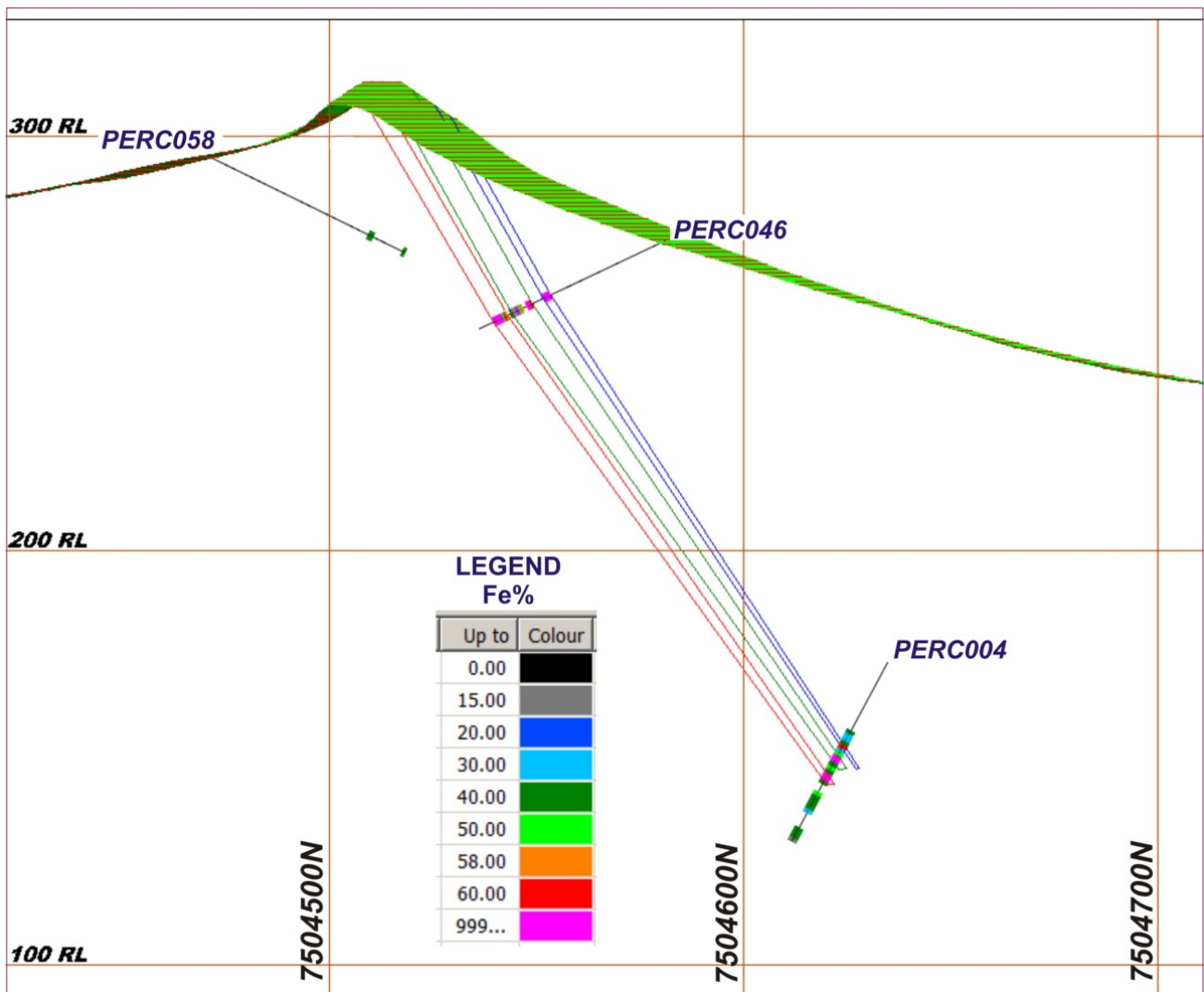
Figure 23: Typical cross section (432285E) showing three main mineralised units
