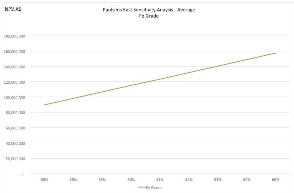
Figure 10: Sensitivity Analysis – Average Fe Grade over LOM (Base Case 61% Fe)
