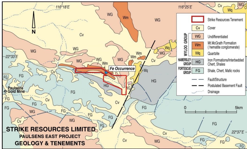
Figure 12: Paulsens East Geology Map
