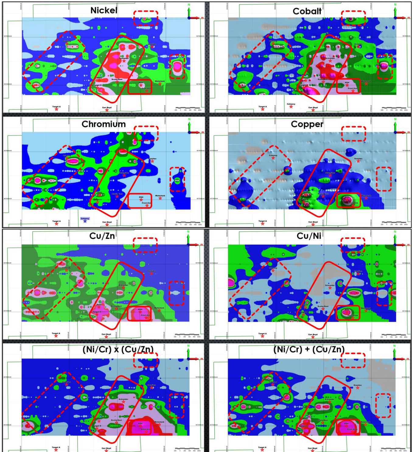
Figure 3: Key elemental and pathfinder vector plots identifying Nickel associated target zones (red rectangles). Primary targets have solid outlines and secondary targets have dashed outlines.
