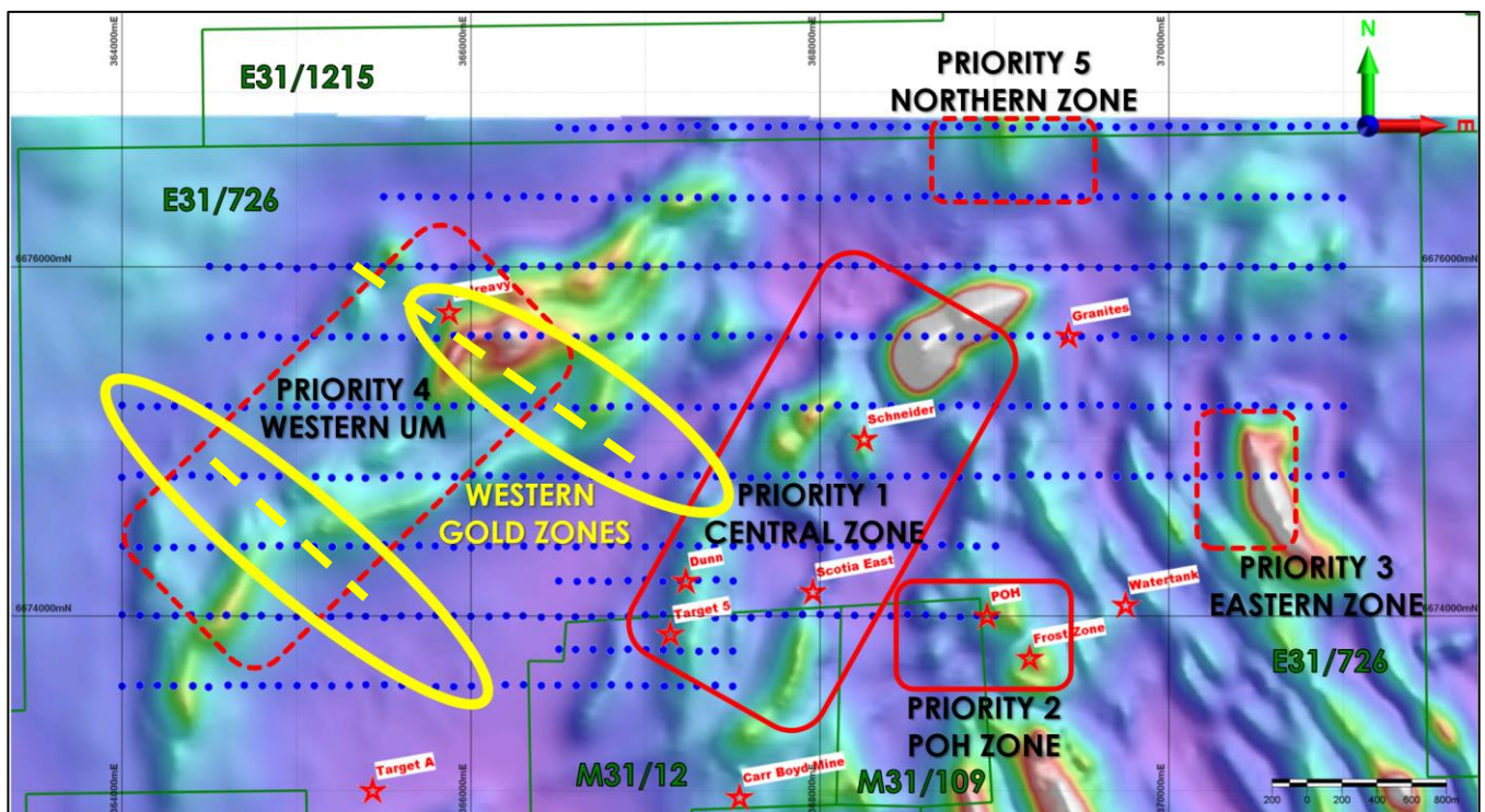
Figure 1. Auger sample sites (blue dots) across Estrella's Carr Boyd Nickel Projects NW tenure. The generated pathfinder Nickel (red) and Gold (yellow) vector target zones are shown over aeromagnetic image (TMI-RTP) along with previously identified prospects.
