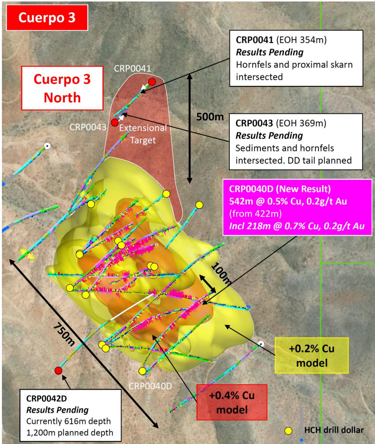
Figure 2 Plan view of Cuerpo 3 - the Main porphyry of the four porphyry centres discovered to date at Cortadera. The plan displays the location of significant new results and pending results from recently completed DD and RC drilling. Note the growing extent of the modelled higher grade copper zone (red wireframe - +0.4% Cu) and the location of open boundaries for growth of the bulk copper envelope at Cortadera (yellow wireframe - +0.2% Cu)
