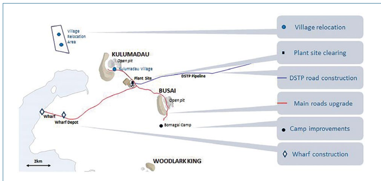
Figure 9: Details of civil works and village relocation activities to be undertaken
