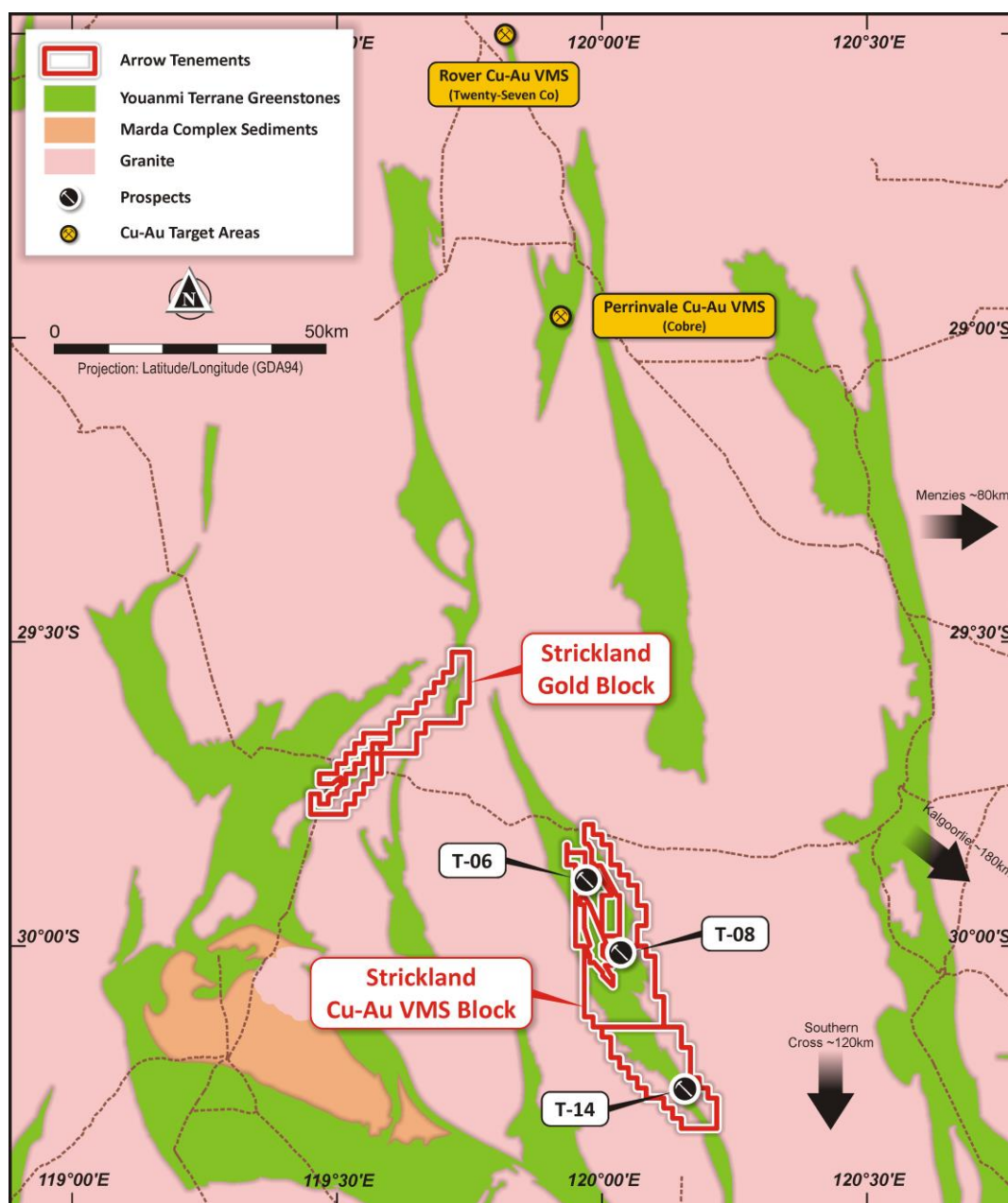
Figure 2: Strickland location map showing geology and Arrow gold and copper-gold tenement blocks with Cu-Au VMS target areas highlighted
