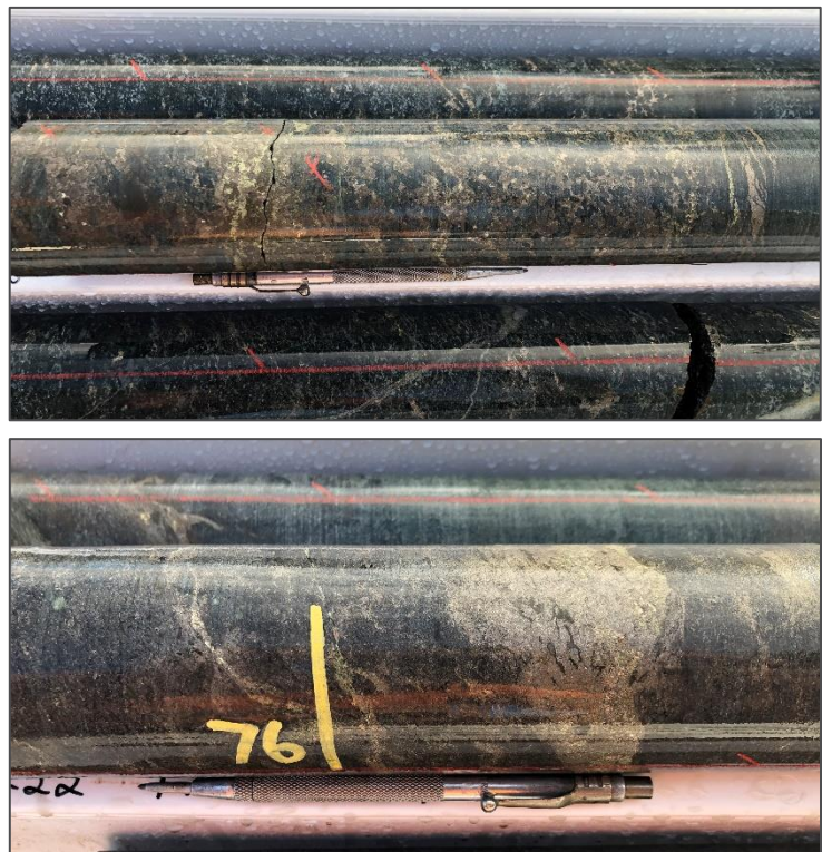
Figure 1. Sulphide mineralisation at 54m depth (top) and 76m in YAD0010 (bottom).
