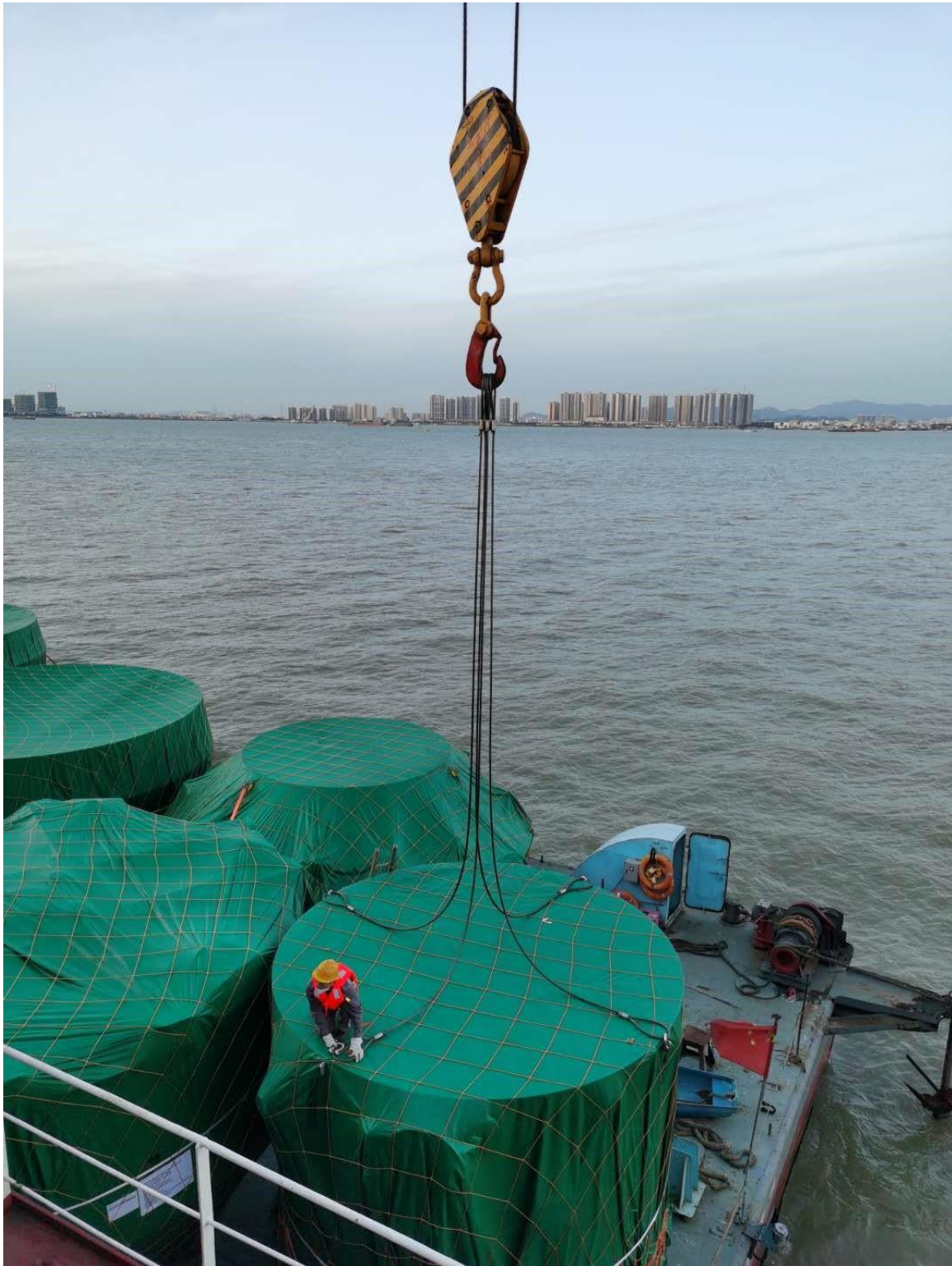
Figure 1: Crystalliser loading onto ship in Guangdong province, China
