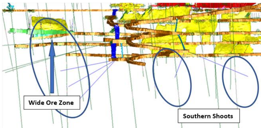
Figure 2 Long section looking East with designed holes in blue.
