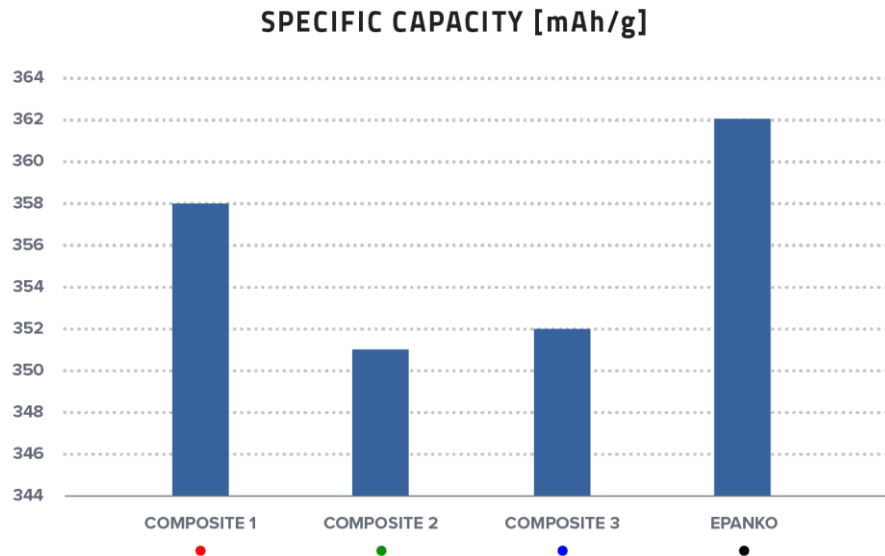
Figure 1 – Benchmark results measuring specific capacity.
