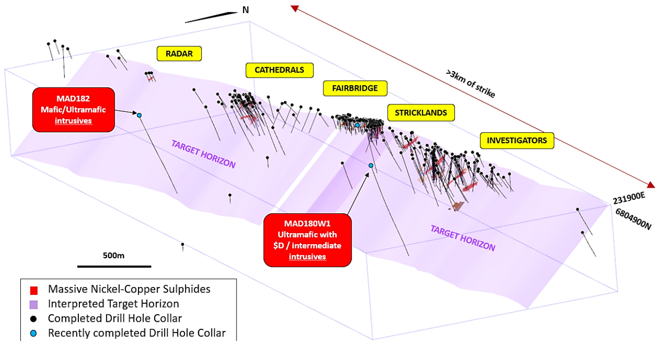
Figure 1 – Schematic orthographic view of the Cathedrals Belt showing the interpreted target horizon, existing drilling and known massive nickel-copper sulphides
