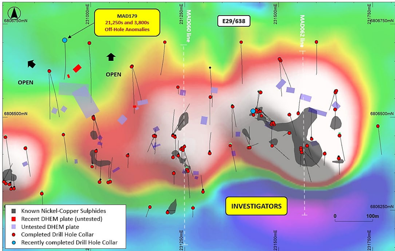
Figure 2 – Plan view of the Investigators Prospect with completed drilling and DHEM plates overlaying SAMSON FLEM image (CH25). The location of MAD179 and the two new EM conductors is highlighted.
