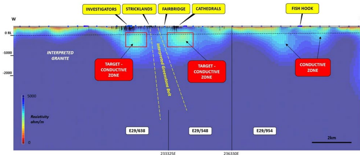
Figure 3 – East-west section (looking north) of the MT/AMT 3D conductivity data across the Cathedrals Belt. The large conductive feature being drilled at Fairbridge is highlighted.
