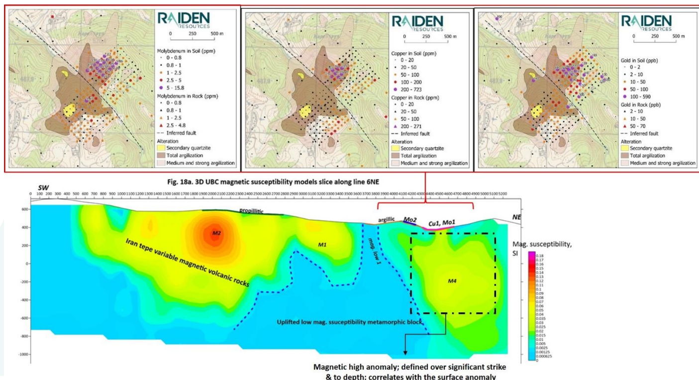
Figure 3 - 3D UBC magnetic susceptibility inversion models over the Sbor prospect depicting the size and vertical extent of the M4 magnetic high, which is interpreted as a potential porphyry related (potassic) alteration zone. The magnetic anomaly at Sbor coincides with the outcropping mineralisation and a well-defined Copper-Gold-Molybdenum soil anomaly
