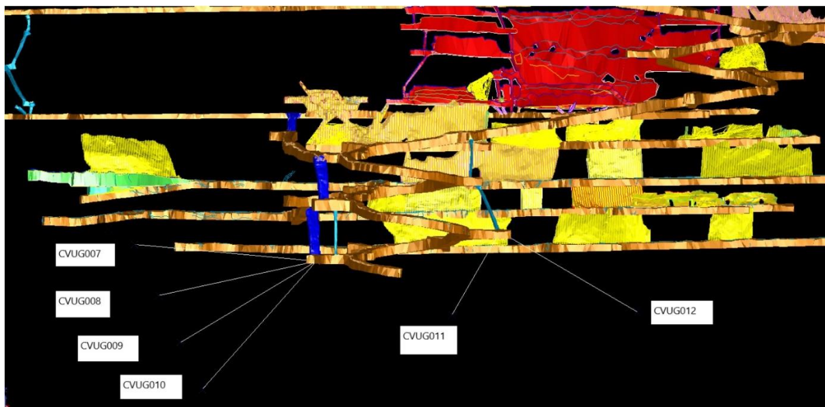
Figure 1 Long section of Comet Vale workings showing spatial relationship of the six-hole program
