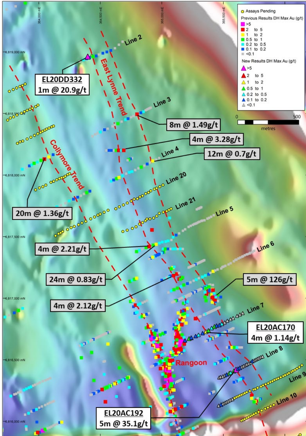
Figure 2: Location of the East Lynne AC drilling program. Results for Line 7 and Line 8 are reported in this announcement and illustrated with white shaded labels. Recent AC and historical RC results are illustrated with grey shaded labels.
