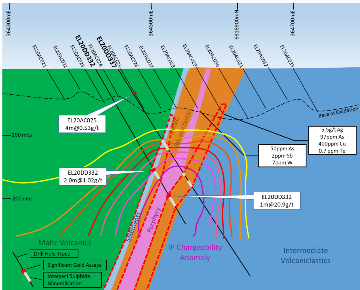
Figure 3: Cross-section of Line 2 East Lynne DD drilling program. Results show zones of strong sulphide mineralisation marked by sporadic high grade gold intersections for EL20DD332. EL20DD337 drilled 40m up-dip shows similar sulphide mineralisation -assays pending. Sulphide mineralisation in both holes explains the coincident strong IP anomaly.
