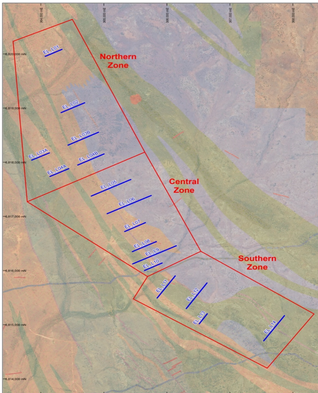
Figure 1: Location of the East Lynne AC and DD drilling program. Air-core results for the Central Zone are reported in this announcement together with initial results for diamond drilling in the Northern Zone.
