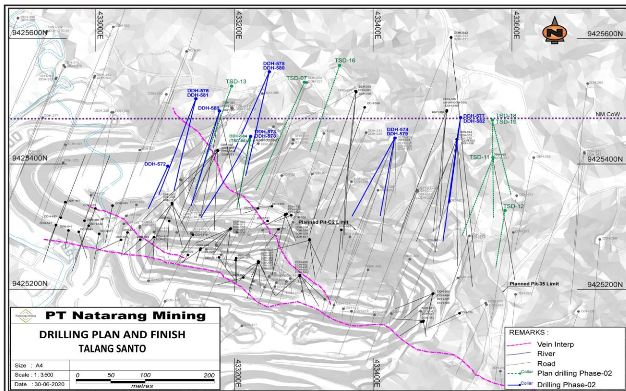
Figure 2. Drill hole locations Phase 2 Talang Santo deep drilling (Completed holes shown in blue).
