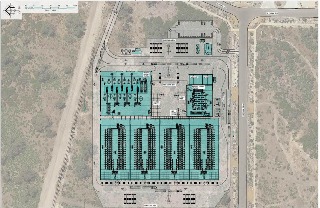
Figure 2 – Site layout of 20,000tpa Manufacturing Facility
