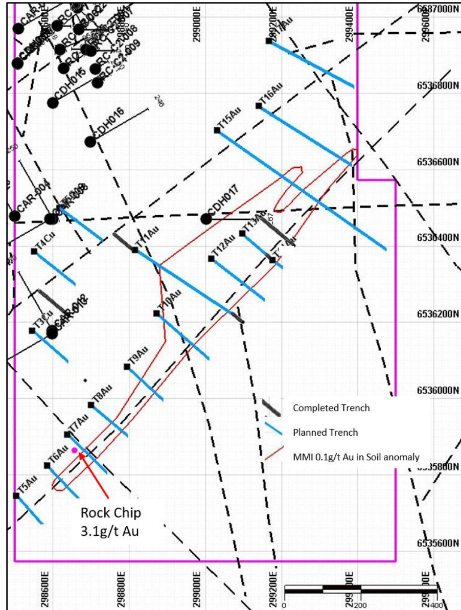
Figure 2: Colina2 planned trench Locations.
