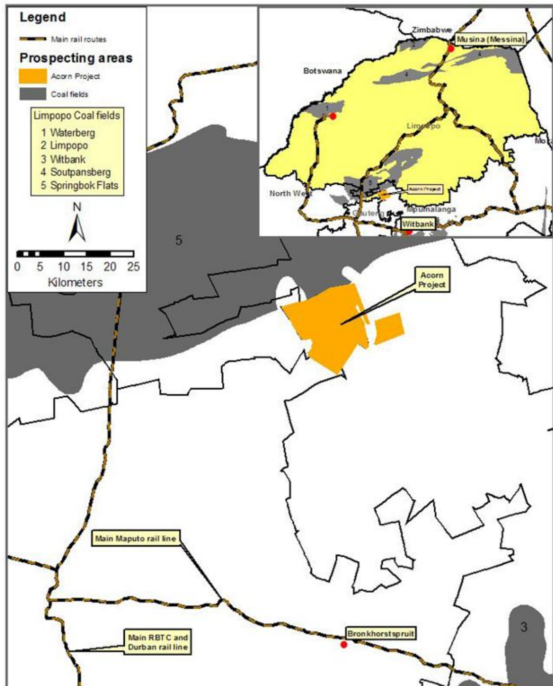
Figure 2: Location of Acorn Project in Mpumalanga, South Africa.
