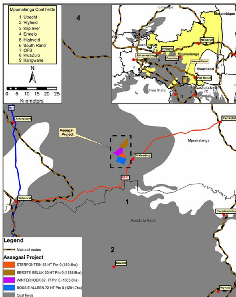
Figure 1: Location of Assegaai Project in Mpumalanga, South Africa.
