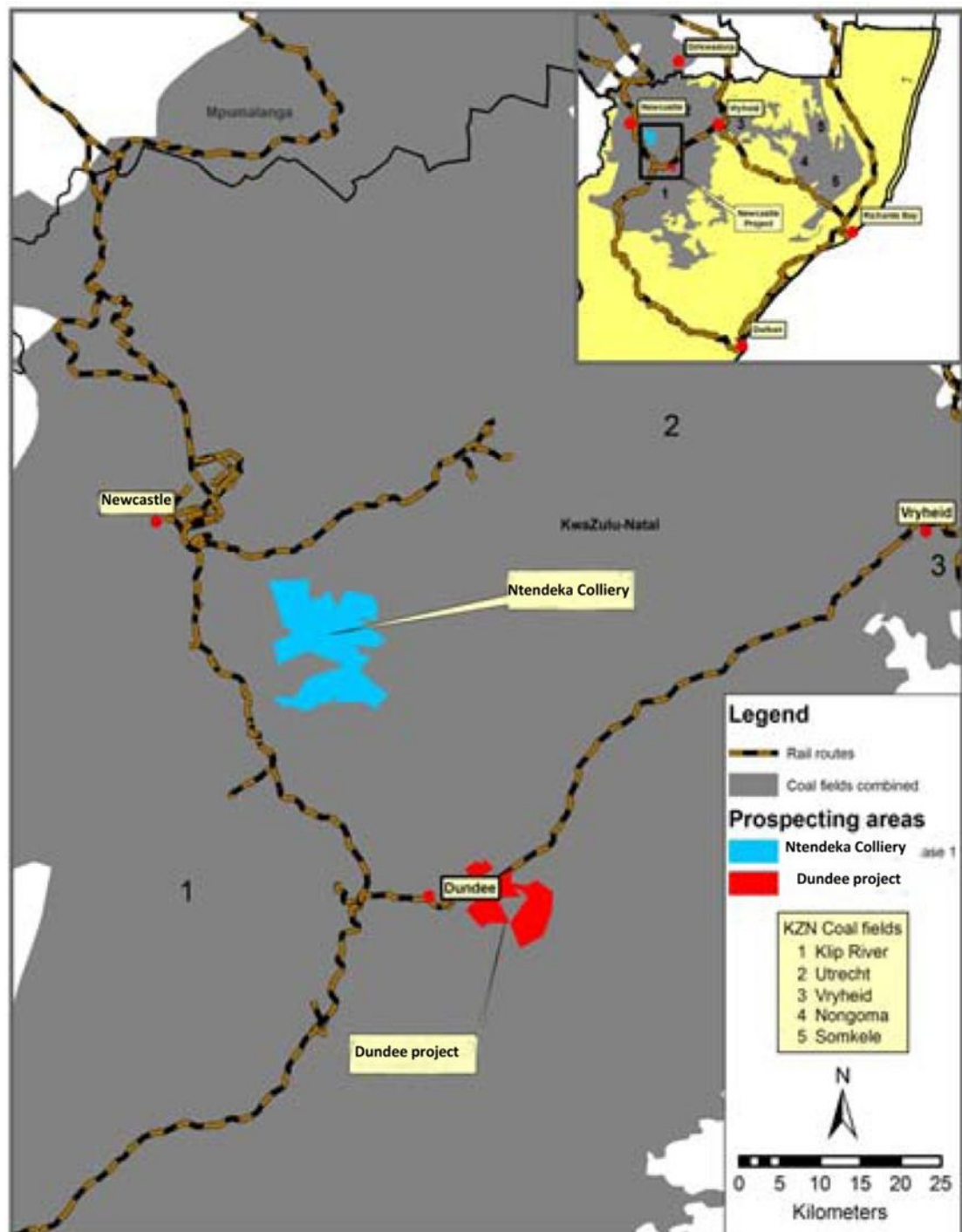
Figure 3: Location of the Dundee Project and Ntendeka Colliery in Kwa-Zulu Natal, South Africa.
