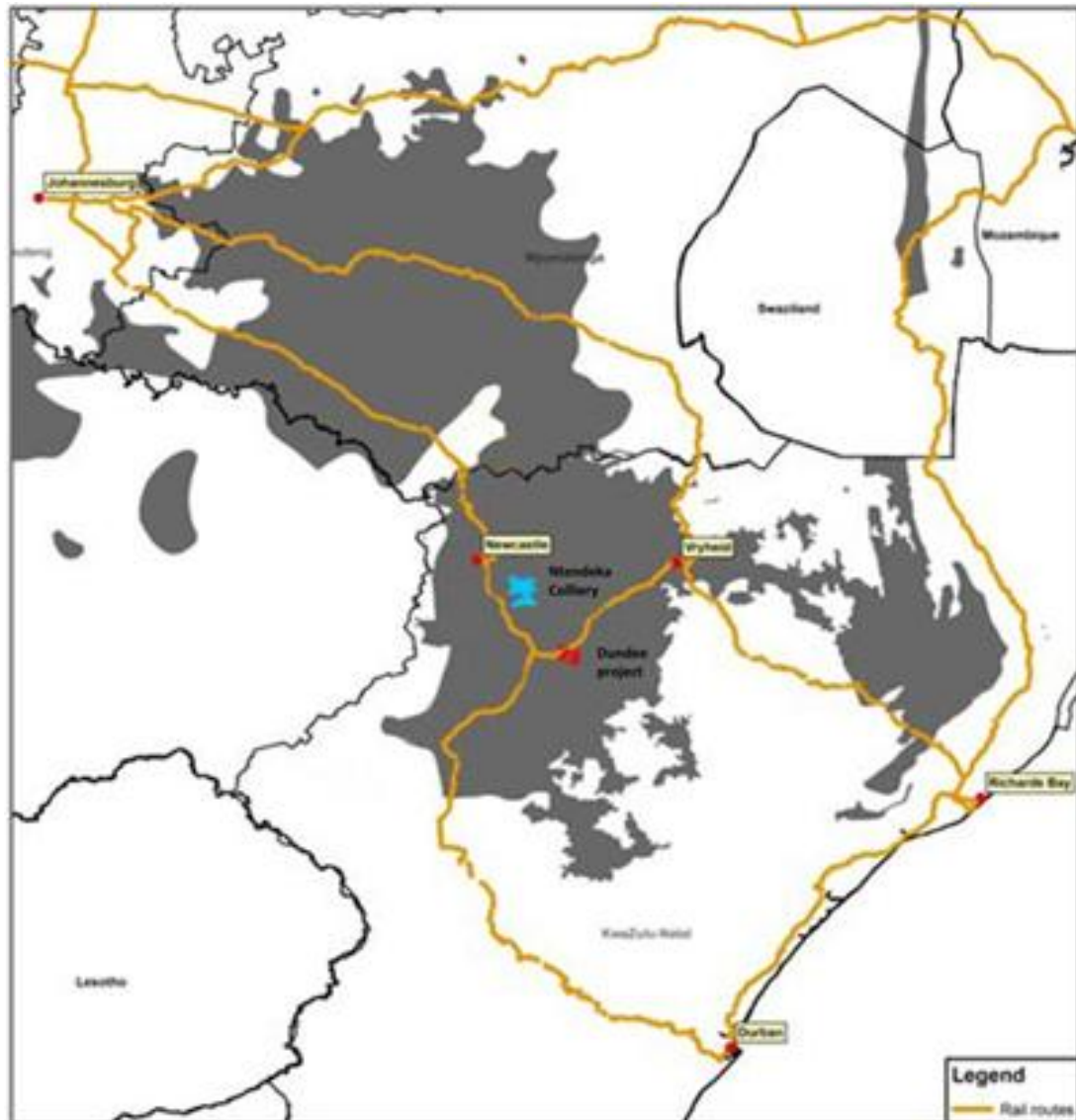
Figure 4: Location of the Dundee Project and Ntendeka Colliery in Kwa-Zulu Natal, South Africa relative to Johannesburg and the ports of Richards Bay and Durban with the main rail lines shown in yellow.
