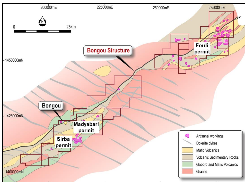
Figure 1: Locality of renewed permits on geology background
