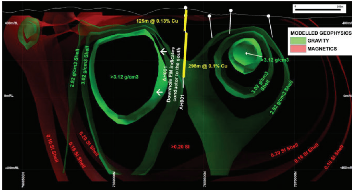
Long Sectional View
