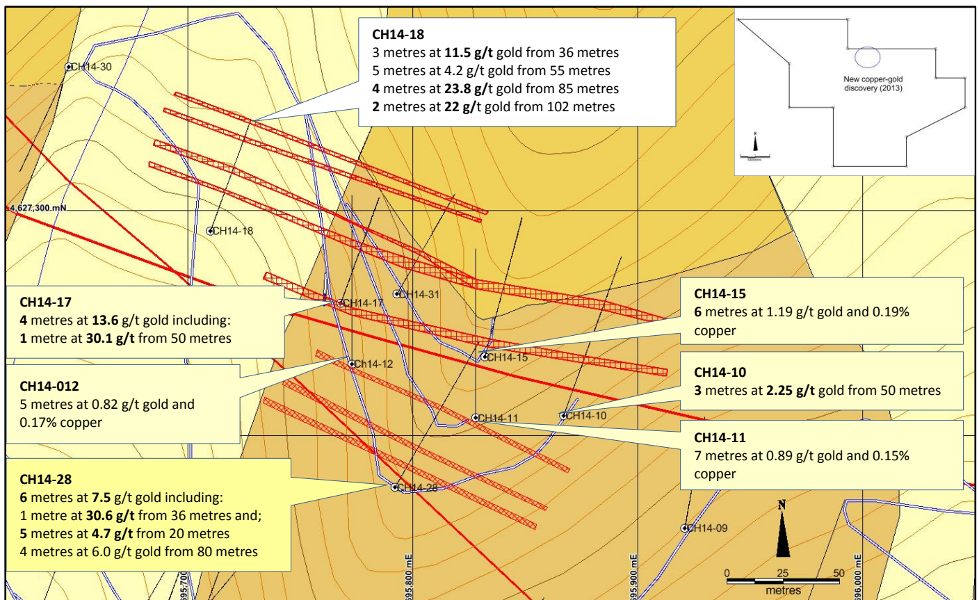
Figure 1 Copper Gold Zone (CGZ) map showing completed drill-hole locations, roads in blue, mineralised zones in red hatch. New results in yellow text box
