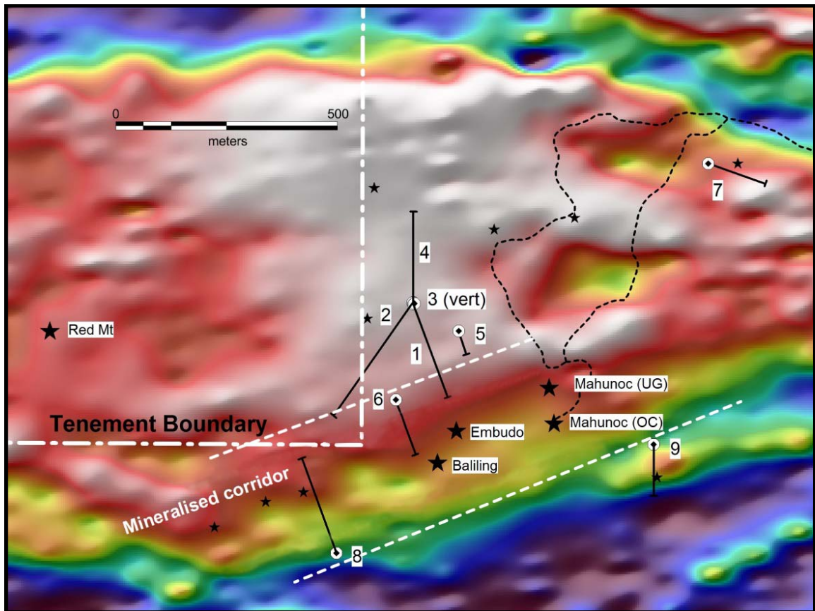
Figure 2 – Drill Hole Locations with Artisanal Workings (marked by black stars) and TMI Ground Magnetic Image of the Mahunoc Diatreme (red and white colours)
