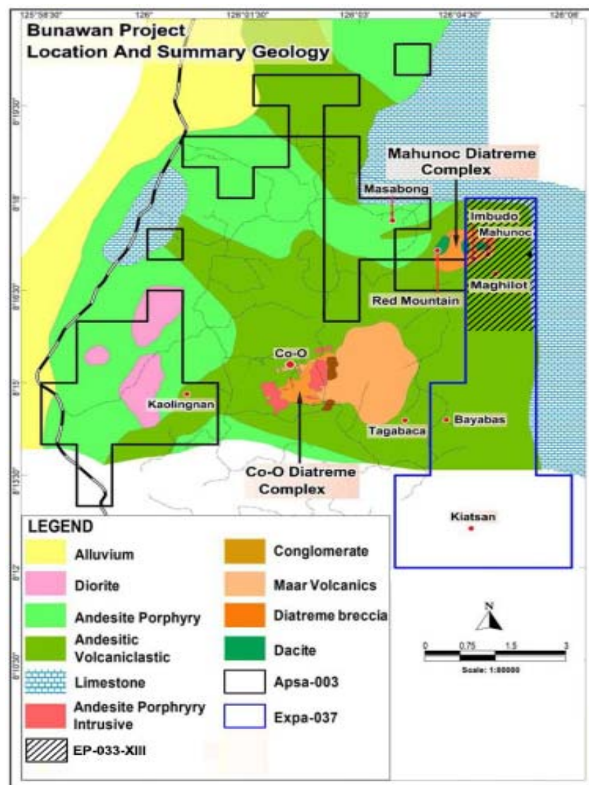
Figure 1 - Location Plan with Regional Geology Showing Both the Co-O and Mahunoc Diatreme Complexes
