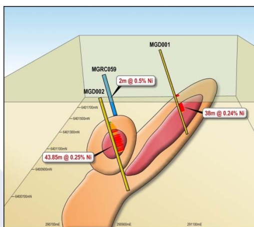
Figure 1: Image showing Hannans' RC drillhole (blue) and the two diamond drillholes recently drilled by Neometals. The orange and red features are modelled magnetic anomalies.
