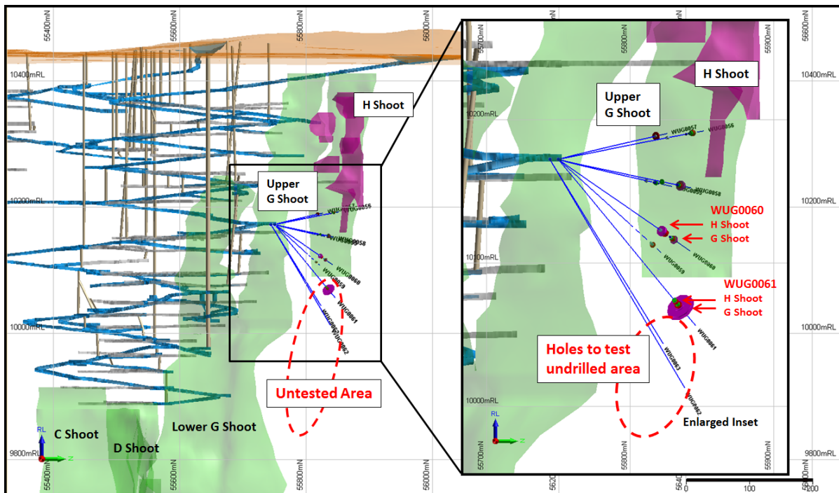
Figure 1: Mt Windarra Long-Section (Looking West) showing location of current JORC Resources (green) and recent drill holes. The enlarged inset shows the positions of the reported intersections and the holes planned to test the extent of mineralisation.
