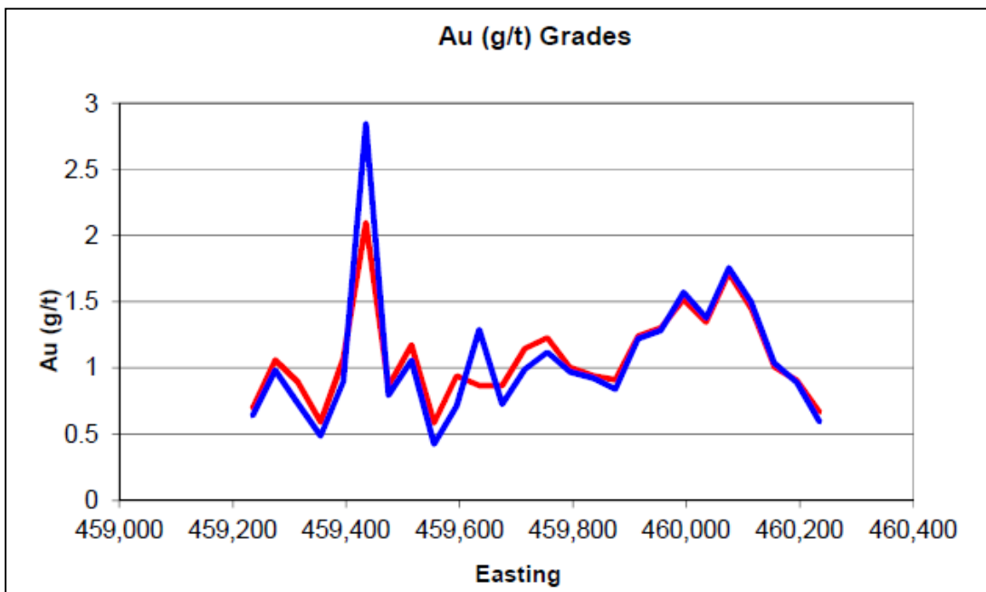
Figure 14-18 Gold Grade Trend Plot by Easting
