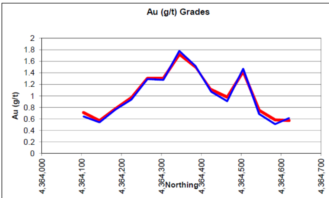
Figure 14-19 Gold Grade Trend Plot by Northing
