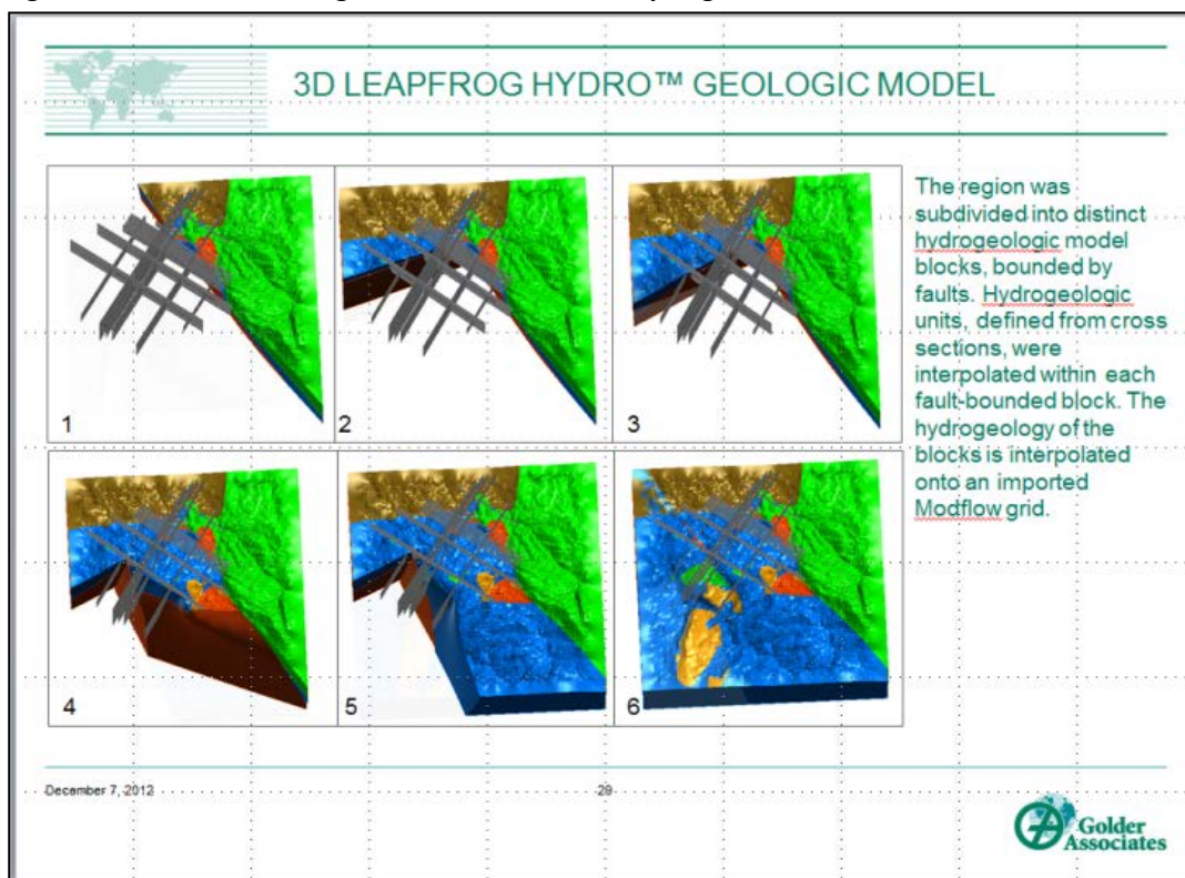
Figure 7-7 Individual Geologic Models Created in Leapfrog
