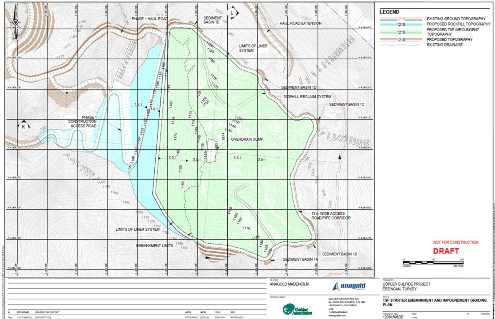
Figure 18-2 TSF Starter Embankment and Impoundment Grading Plan
