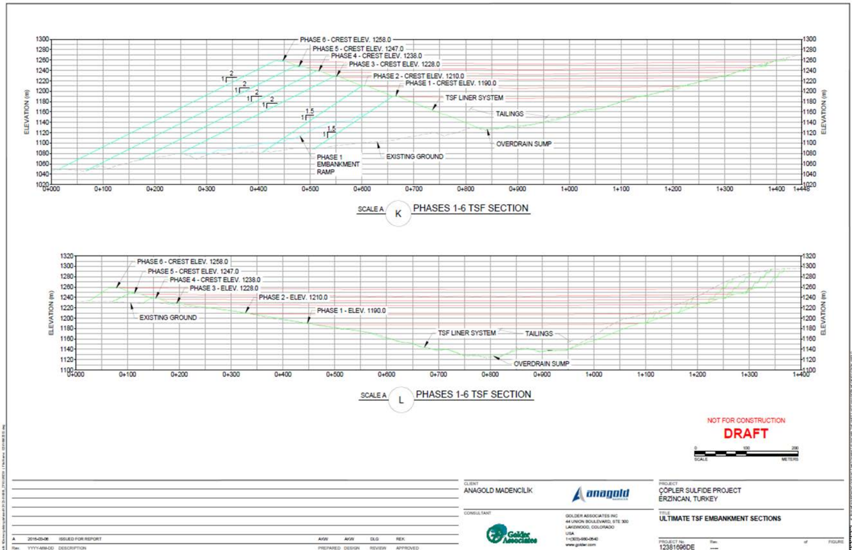
Figure 18-4 TSF Ultimate Embankment Profile
