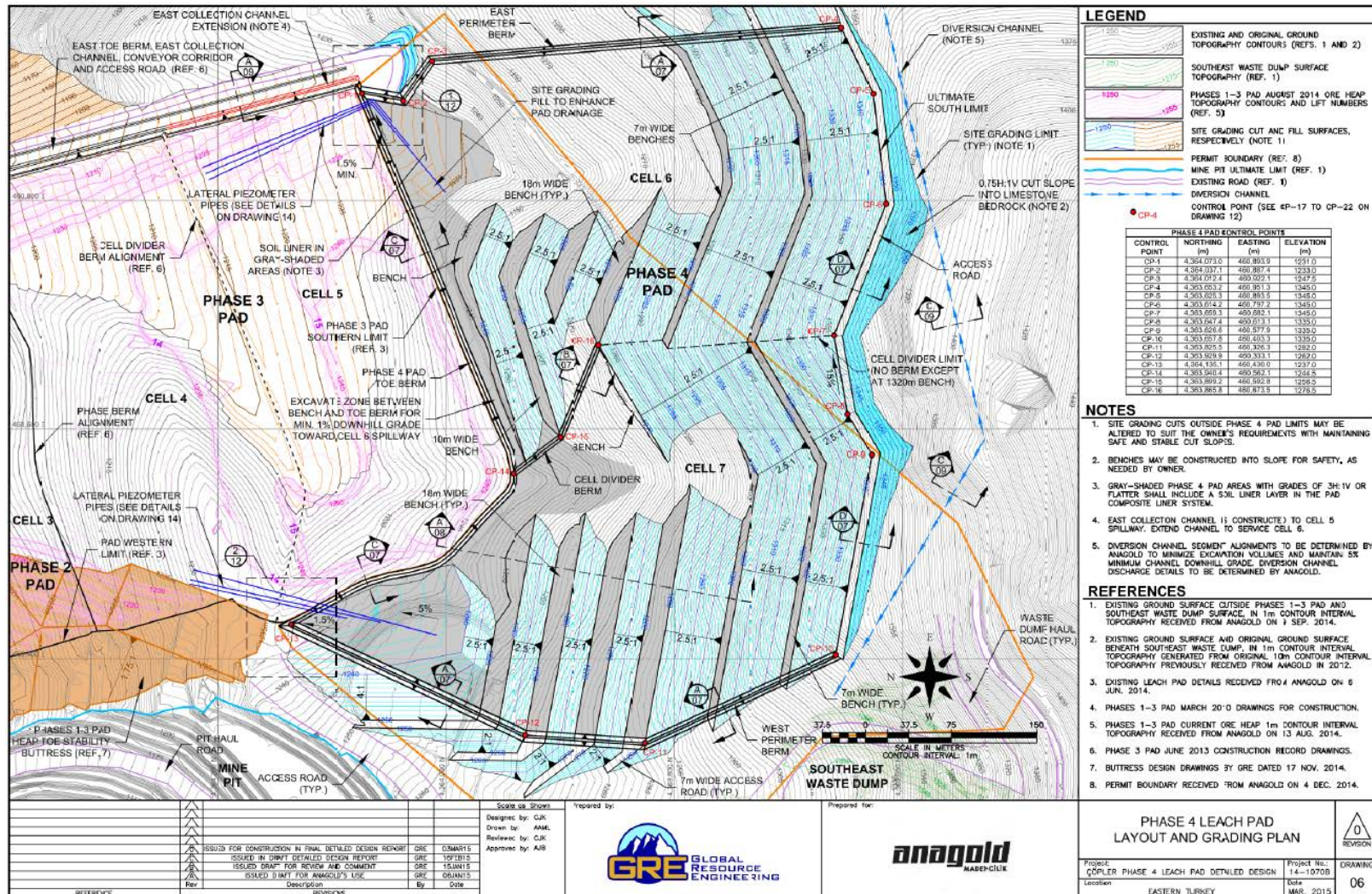
Figure 18-1 Phase 4 Leach Pad Layout and Grading Plan
