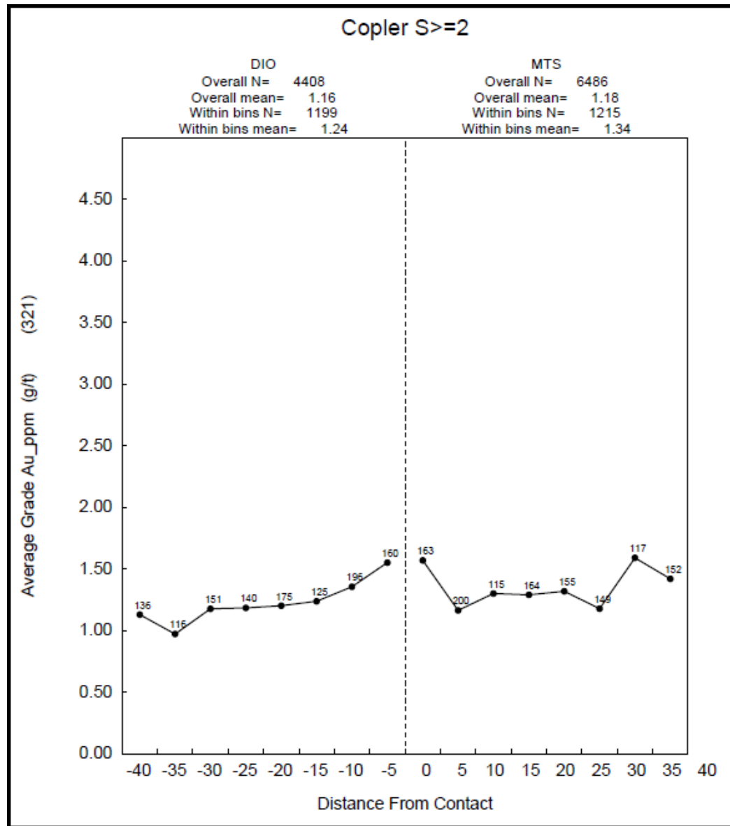
Figure 14-8 Contact plot of Gold across the Diorite–Metasediments Contact for Sulfide Material
