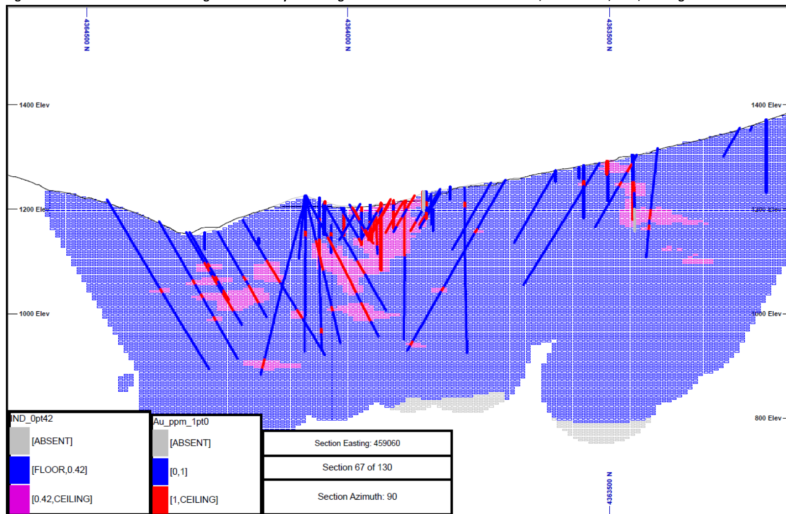
Figure 14-13 Cross Section illustrating the Geometry of the High-Grade Gold Indicator PACK Model; Section 459,060E, looking East
