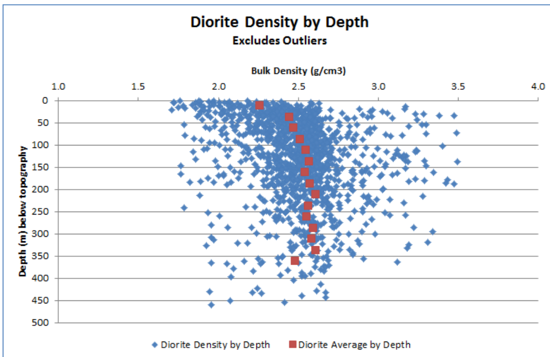
Figure 14-16 Diorite Bulk Density Values by Depth below Surface
