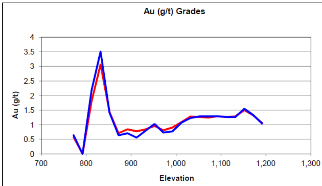
Figure 14-20 Gold Grade Trend Plot by Elevation
