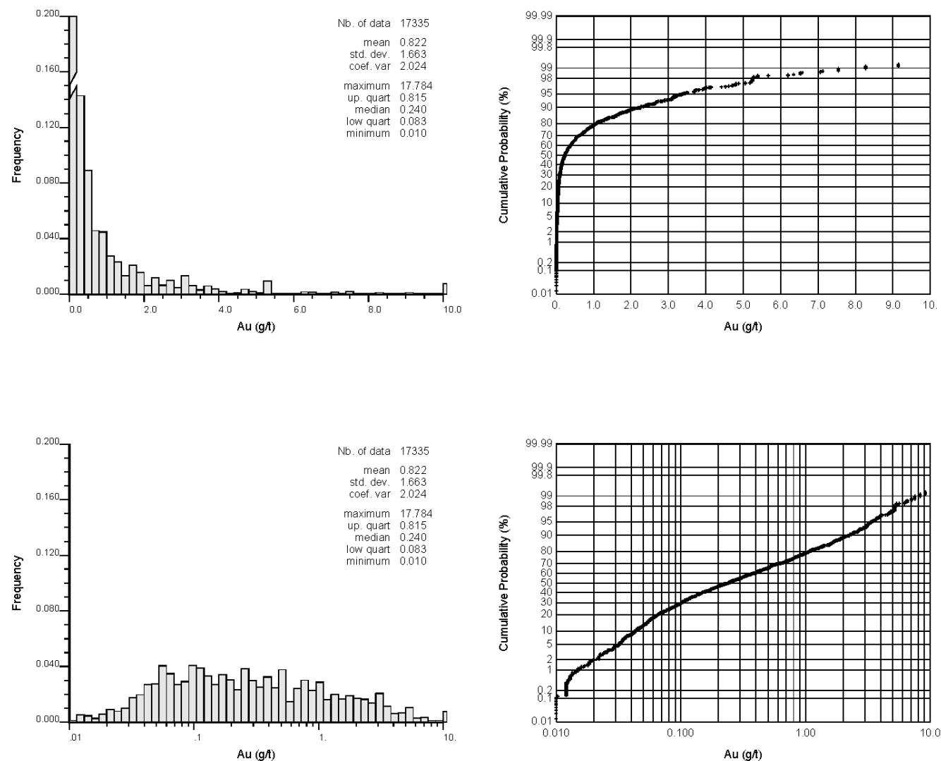
Figure 12-2 Histogram of 10m OMAC Composites
