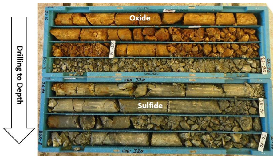
Figure 14-22 Drill Core Photograph Showing Color Change from Oxide to Sulfide
