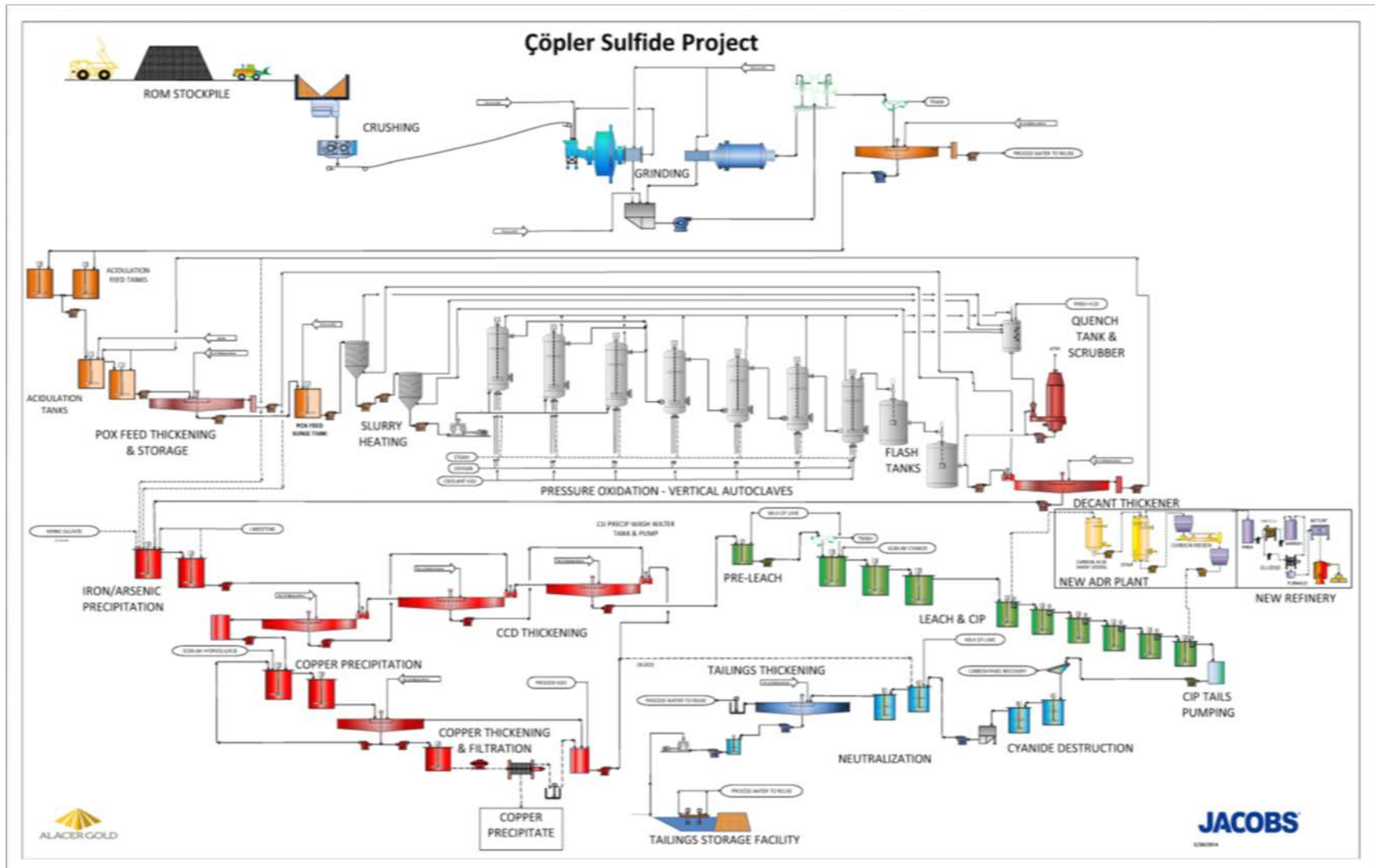
Figure 17-2 Çöpler Sulfide Process Schematic
