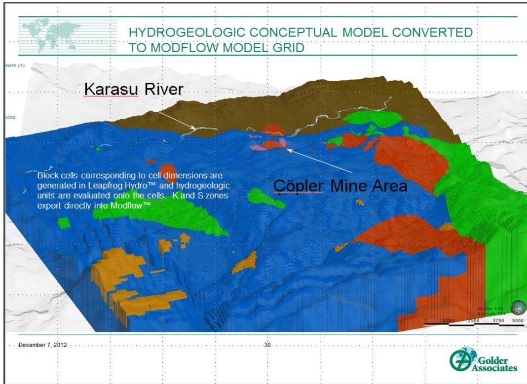
Figure 7-8 Hydrogeologic Model with MODFLOW Grid and Layering
