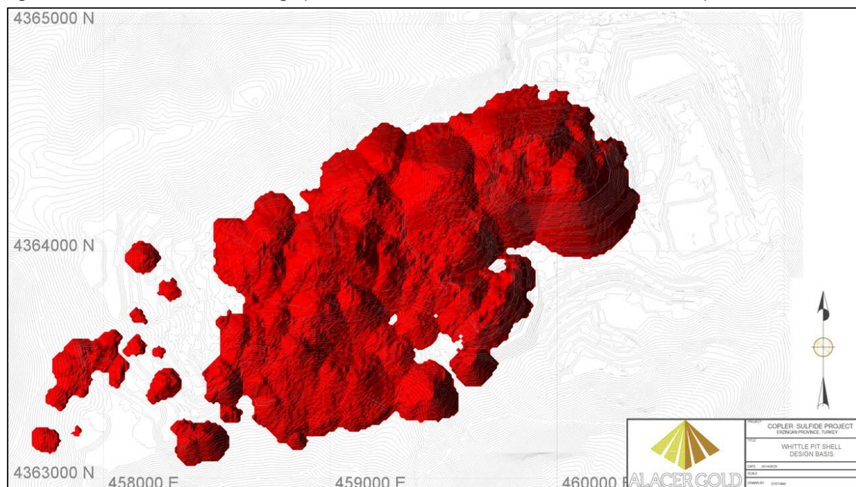
Figure 16-3 Whittle Pit Shell for Design (Oxide Cut-off: BE, Sulfide Cut-off: 1.5, Pit 10-$950Au)
