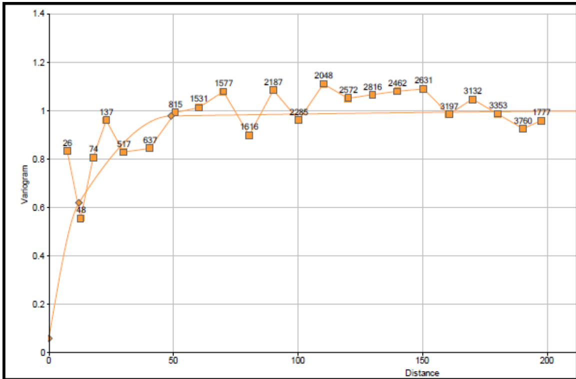
Figure 14-10 Example Gold Variogram for Marble Domain, < 2% S
