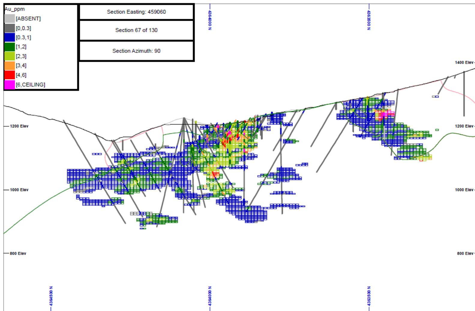
Figure 14-14 Cross Section Illustrating the Combined Low- and High-Grade PACK Gold Estimates; Section 459,060E, looking East
