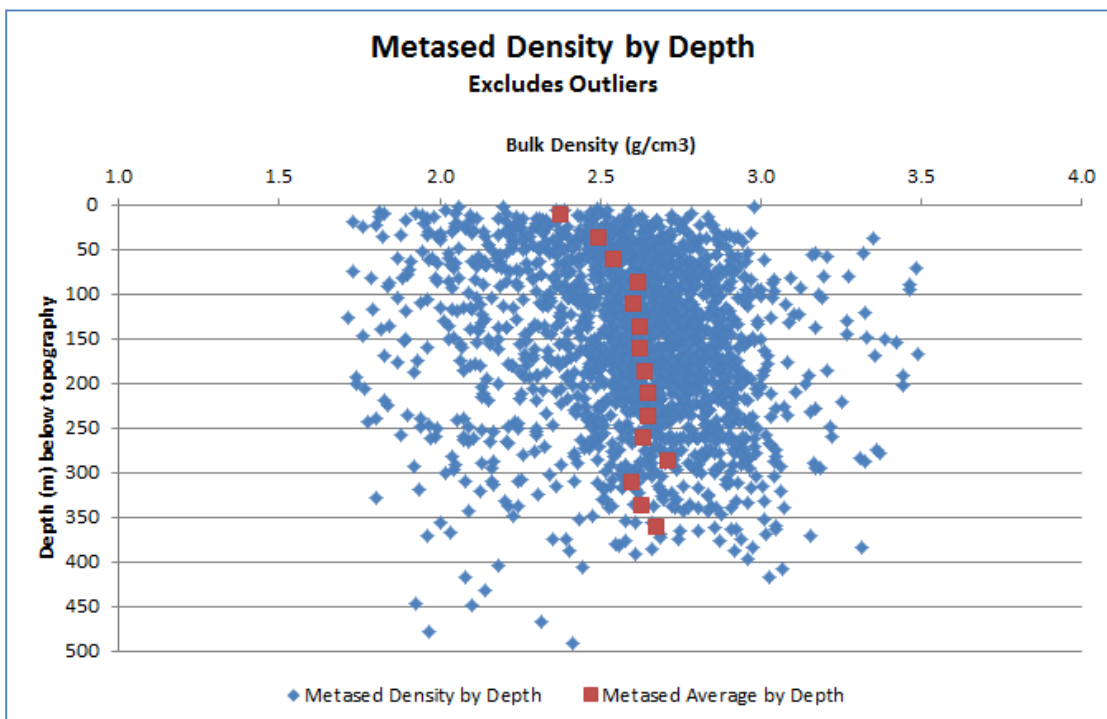
Figure 14-17 Metasediments Bulk Density Values by Depth below Surface
