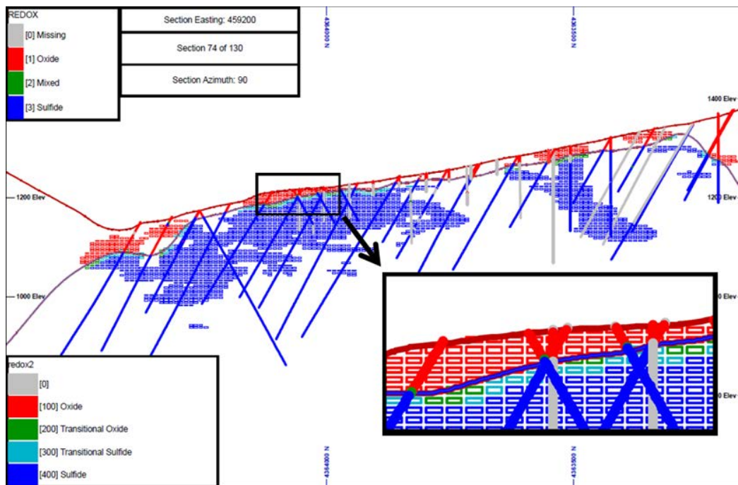
Figure 14-24 Model of the Oxidation Boundaries, Top Left Legend Oxidation Codes for Drill Holes, Bottom Left Legend are Oxidation Codes for Block Model
