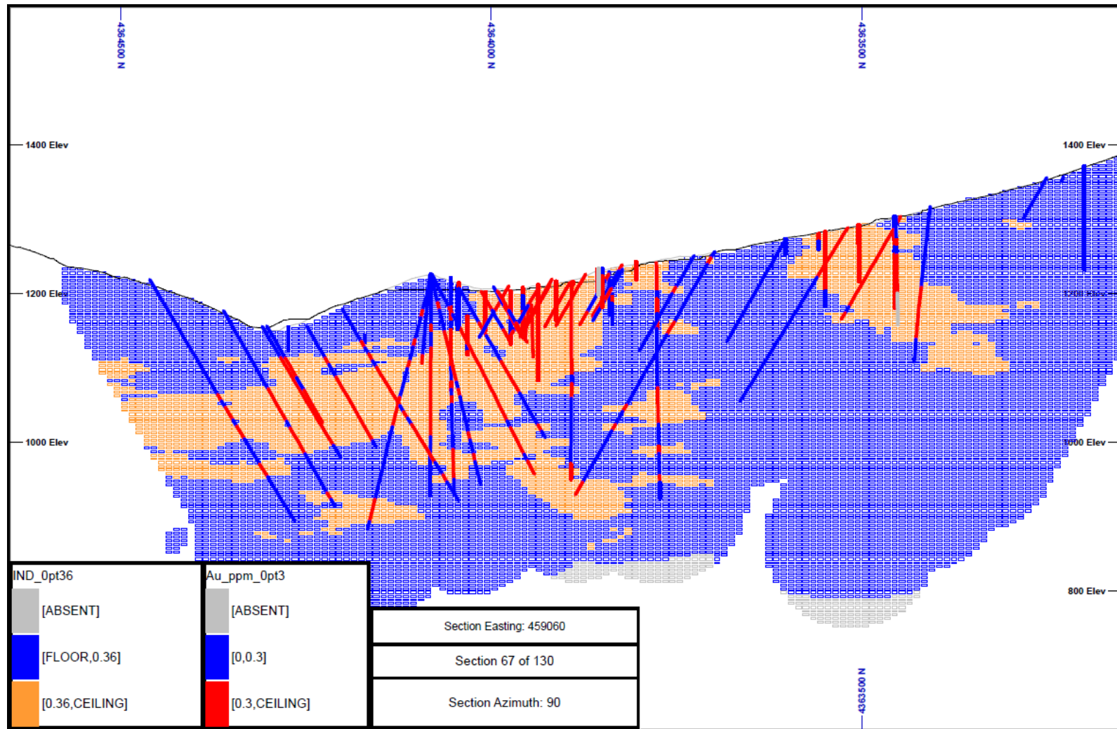
Figure 14-12 Cross Section Illustrating the Geometry of the Low-Grade Gold Indicator PACK Model; Section 459,060E, looking East
