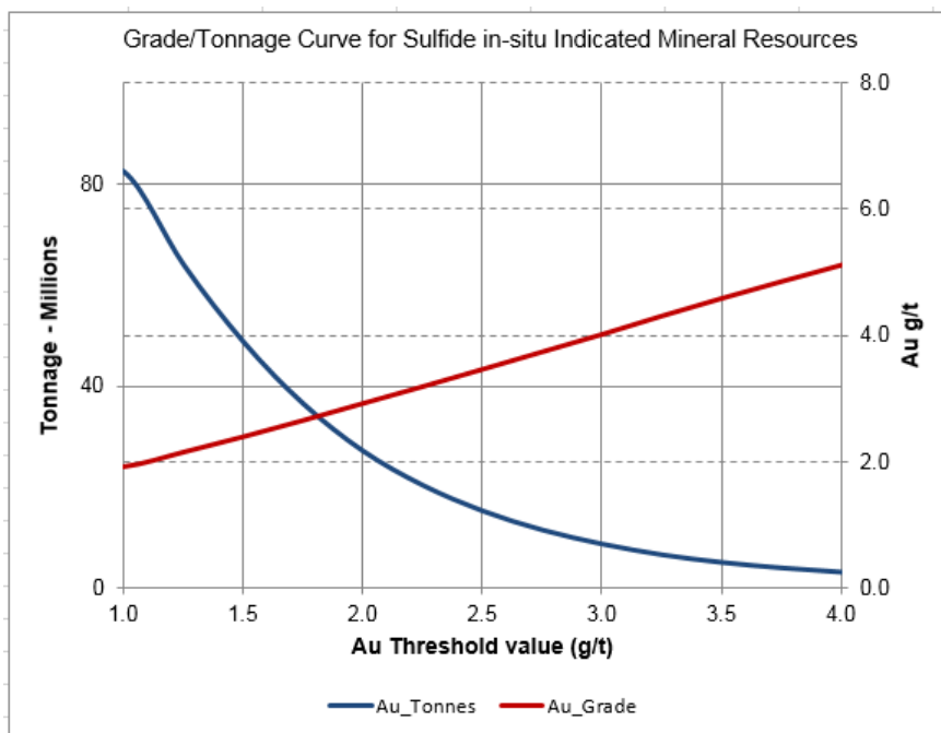
Figure 14-27 Distribution Curve for Sulfide Material Classified as Indicated Mineral Resources within the 2015 Lerchs-Grossmann Conceptual Pit Shell
