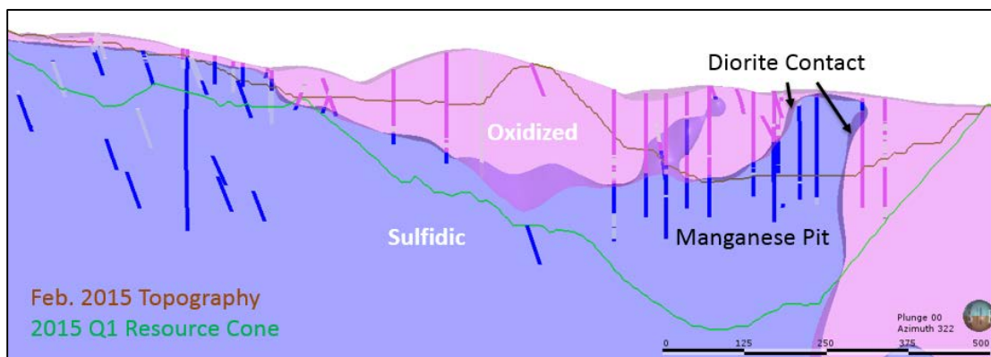
Figure 14-25 Oblique Section plot of the Oxidation Boundary, looking northwest
