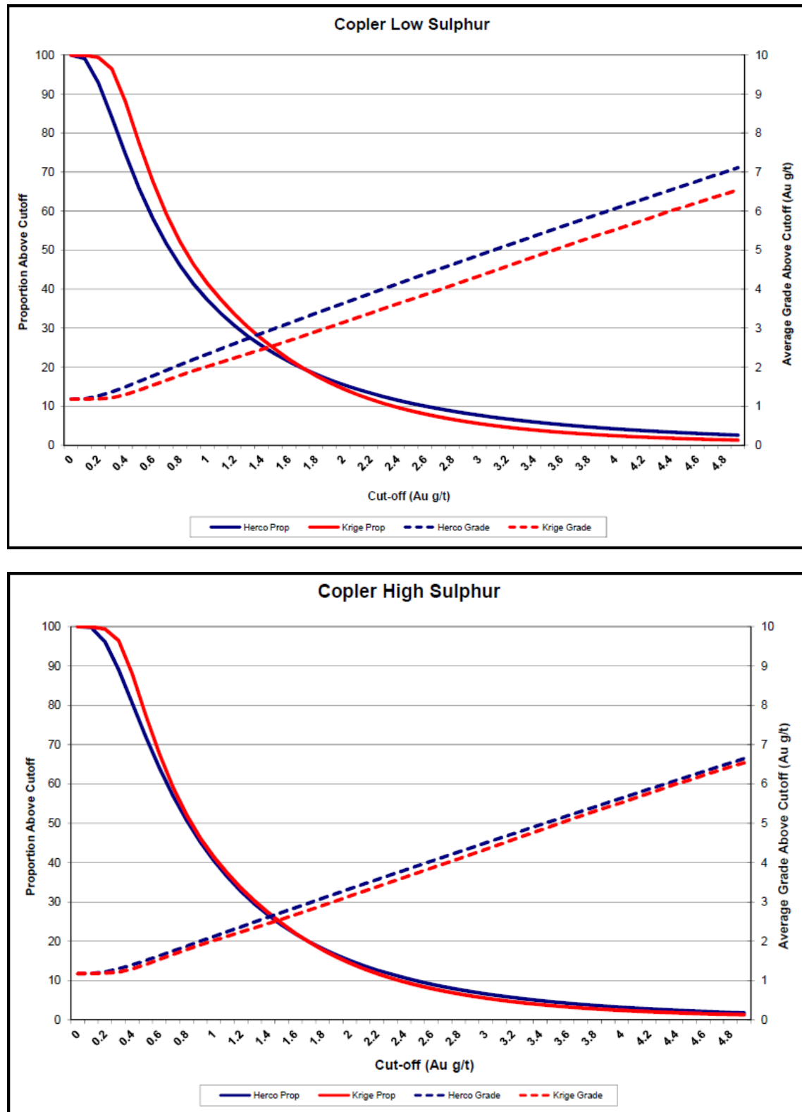
Figure 14-21 Herco Plots Categorized by Low (<2% S) and High (>=2%) Sulfur Content
