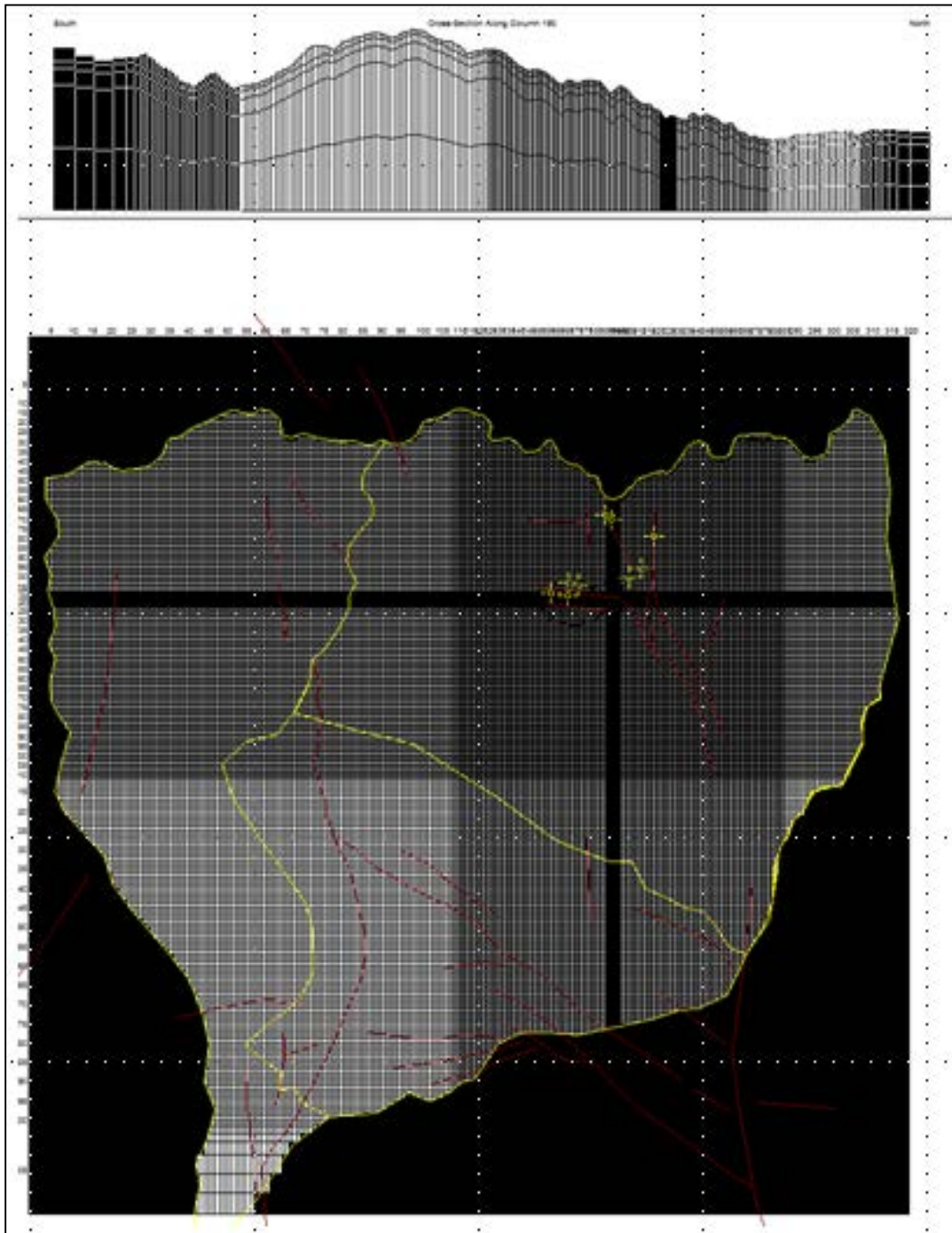
Figure 7-9 Cross Section and Plan View of Model Domain with MODFLOW Grid and Layers
