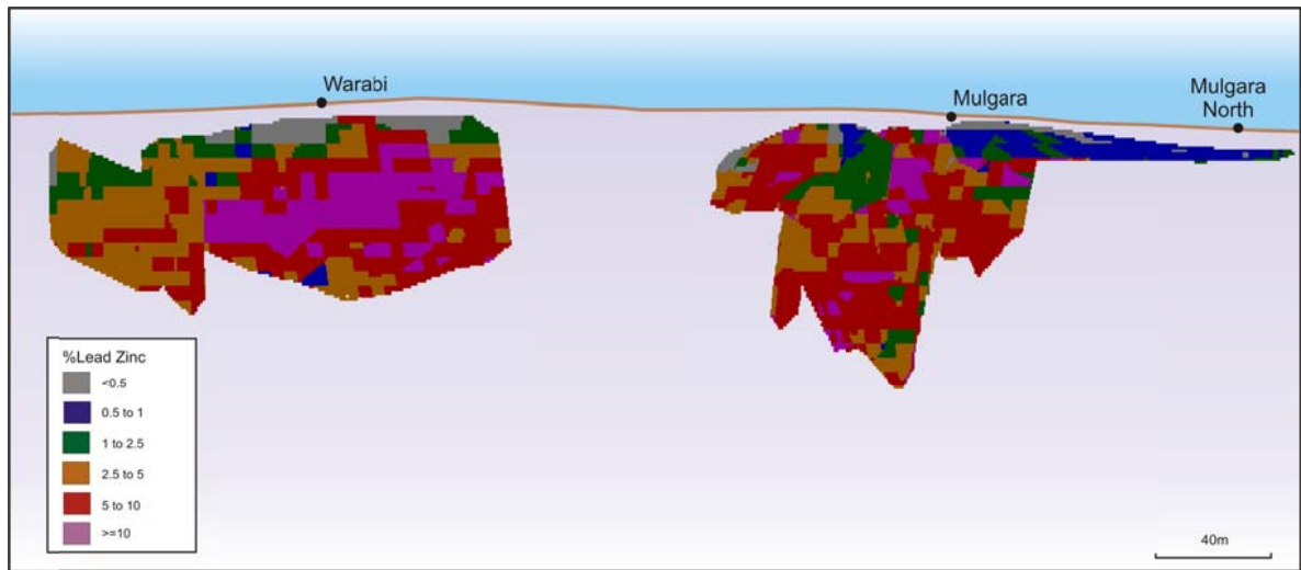
Figure 1 - Long section view of the Warabi (left) and Mulgara (right) mineral resource block models looking south west
