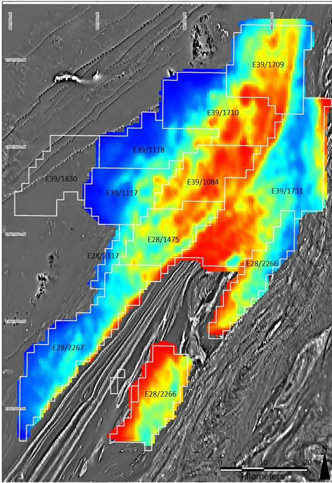
Figure 1 – Regional ground gravity survey 1VD (colour) over regional aeromagnetic TMI 1VD (grey)
