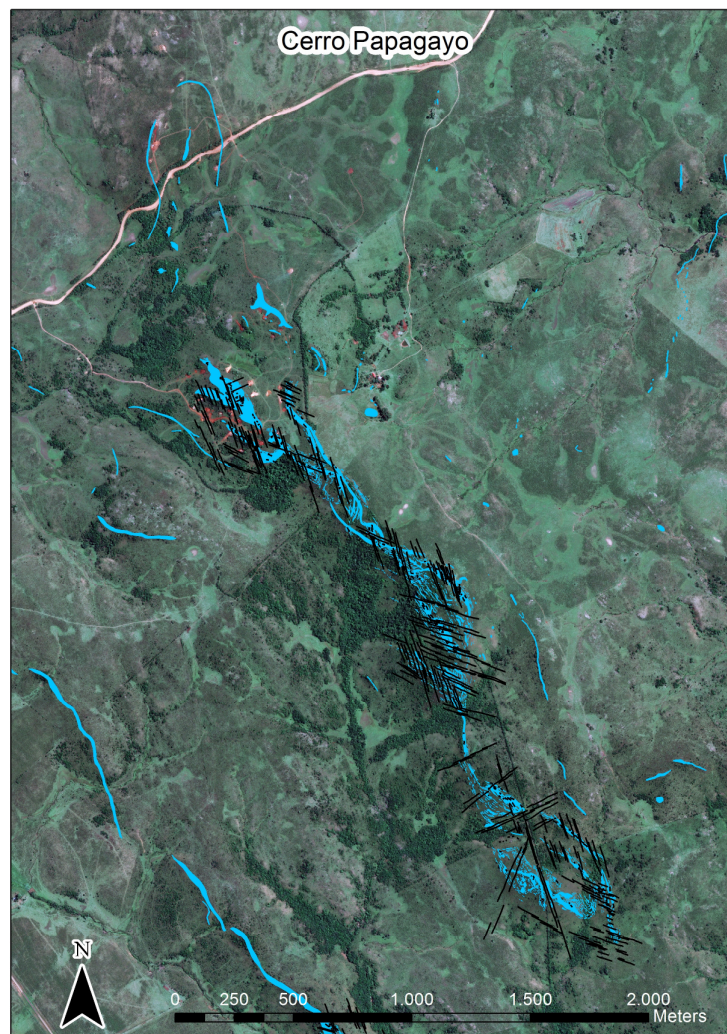
Figure 4: Detail field mapping (1:5000) in Cerro Papagayo.
