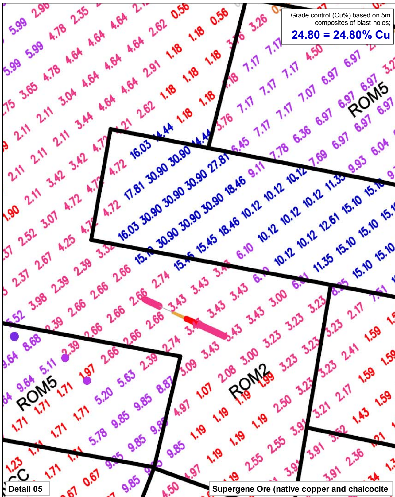
Figure 11: Detail enlargement of grade control results (Cu%) based on 5m composites of blast-hole sampling (eg. 24.80 = 24.80% Cu)...see Figure 8 (master dig-plan) for reference.
