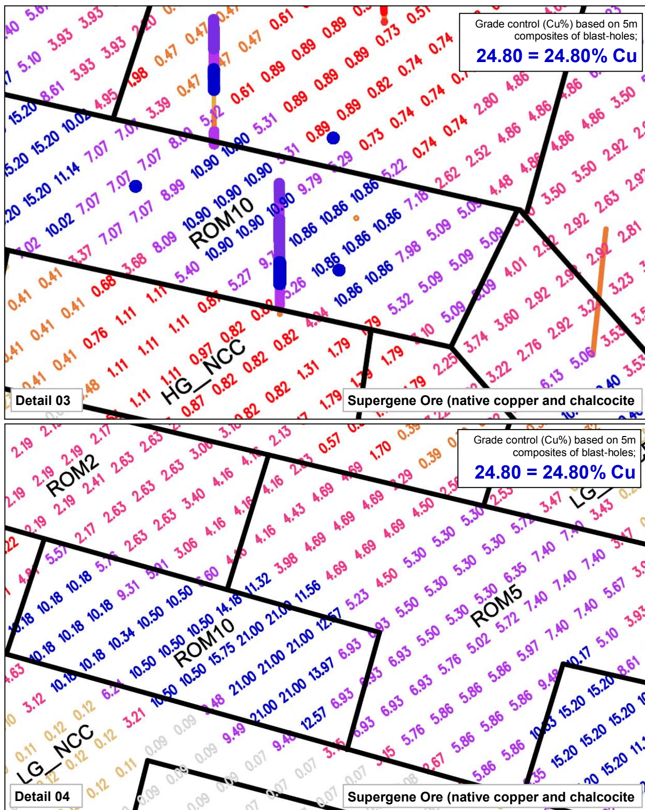
Figure 10: Detail enlargement of grade control results (Cu%) based on 5m composites of blast-hole sampling (eg. 24.80 = 24.80% Cu)...see Figure 8 (master dig-plan) for reference.
