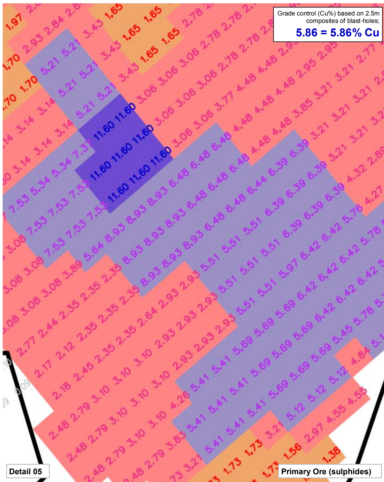
Figure 17: Details of grade-control results for LM2 Pit at RL190 (2.5m composite) in the primary ore...see Figure 14 for master plan.
