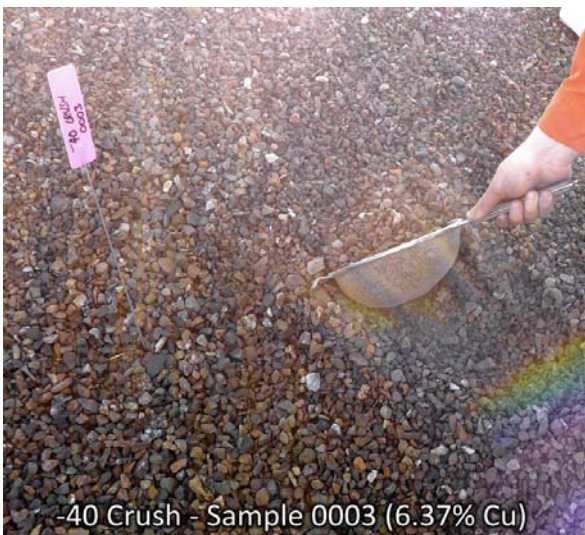
Figure 6: Crushed ore stockpiles (-40mm) grades are estimated from a combination of lab-assay of composite blast-hole samples and where not available, resource grade estimates are used. Check assays are regularly conducted for QAQC purposes.
