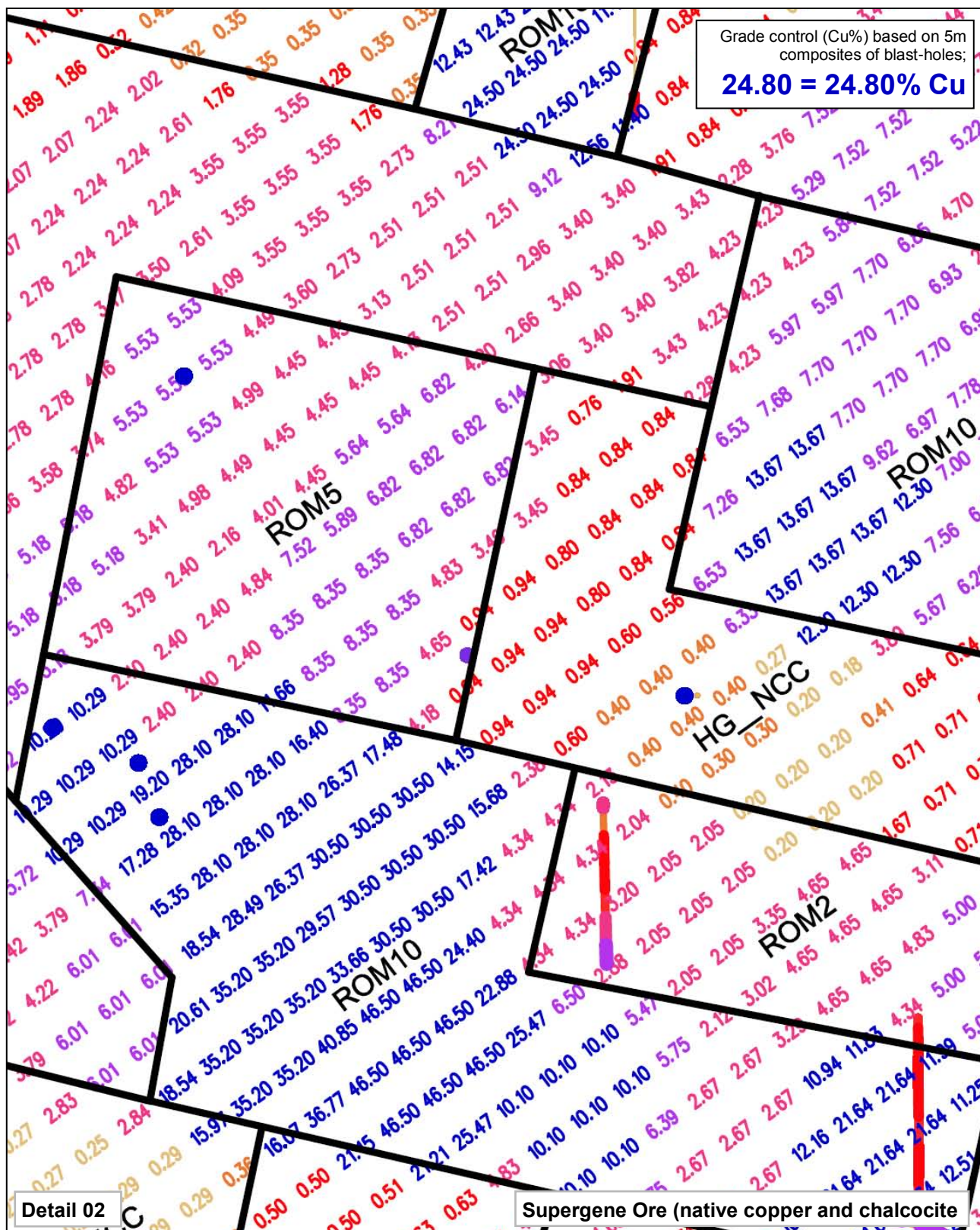
Figure 9: Detail enlargement of grade control results (Cu%) based on 5m composites of blast-hole sampling (eg. 24.80 = 24.80% Cu)...see Figure 8 (master dig-plan) for reference.
