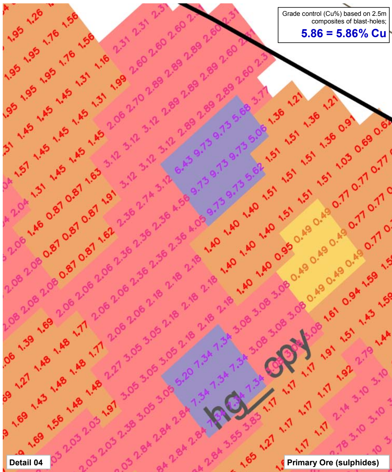
Figure 16: Details of grade-control results for LM2 Pit at RL190 (2.5m composite) in the primary ore...see Figure 14 for master plan.
