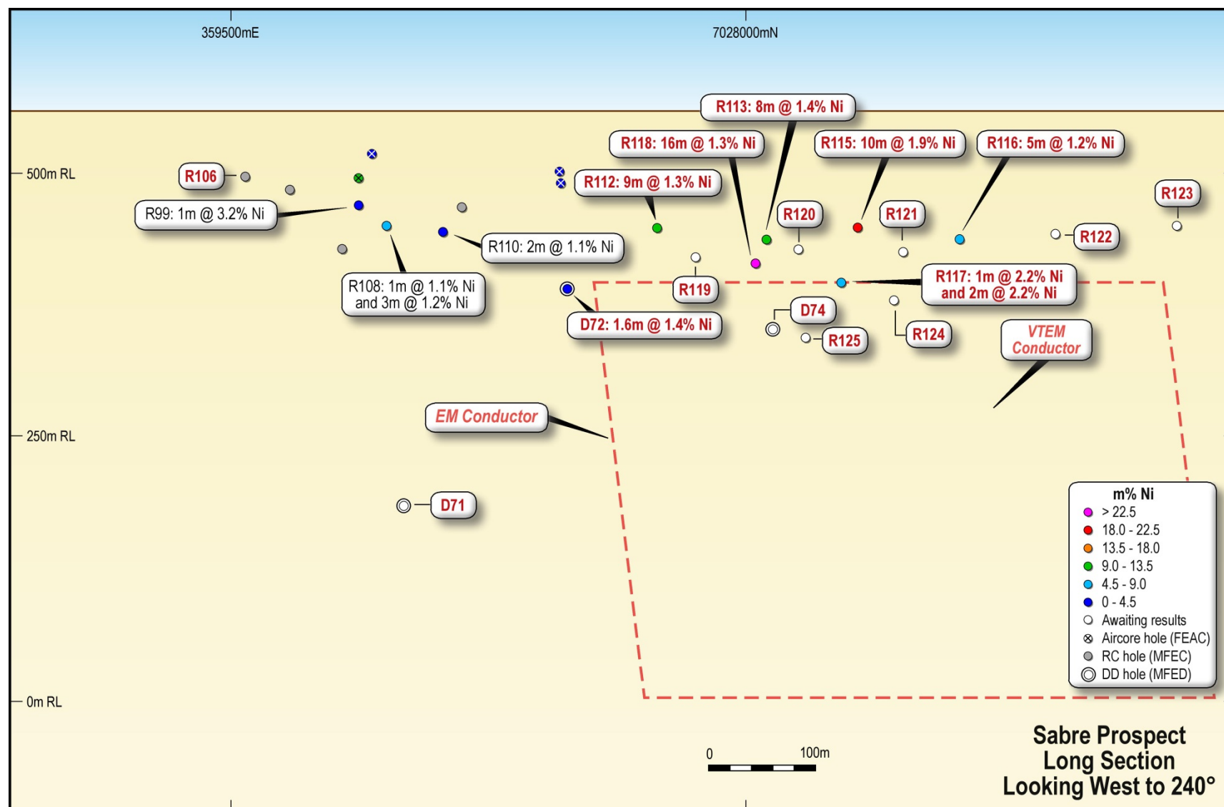
Figure 2: Sabre Long Section
